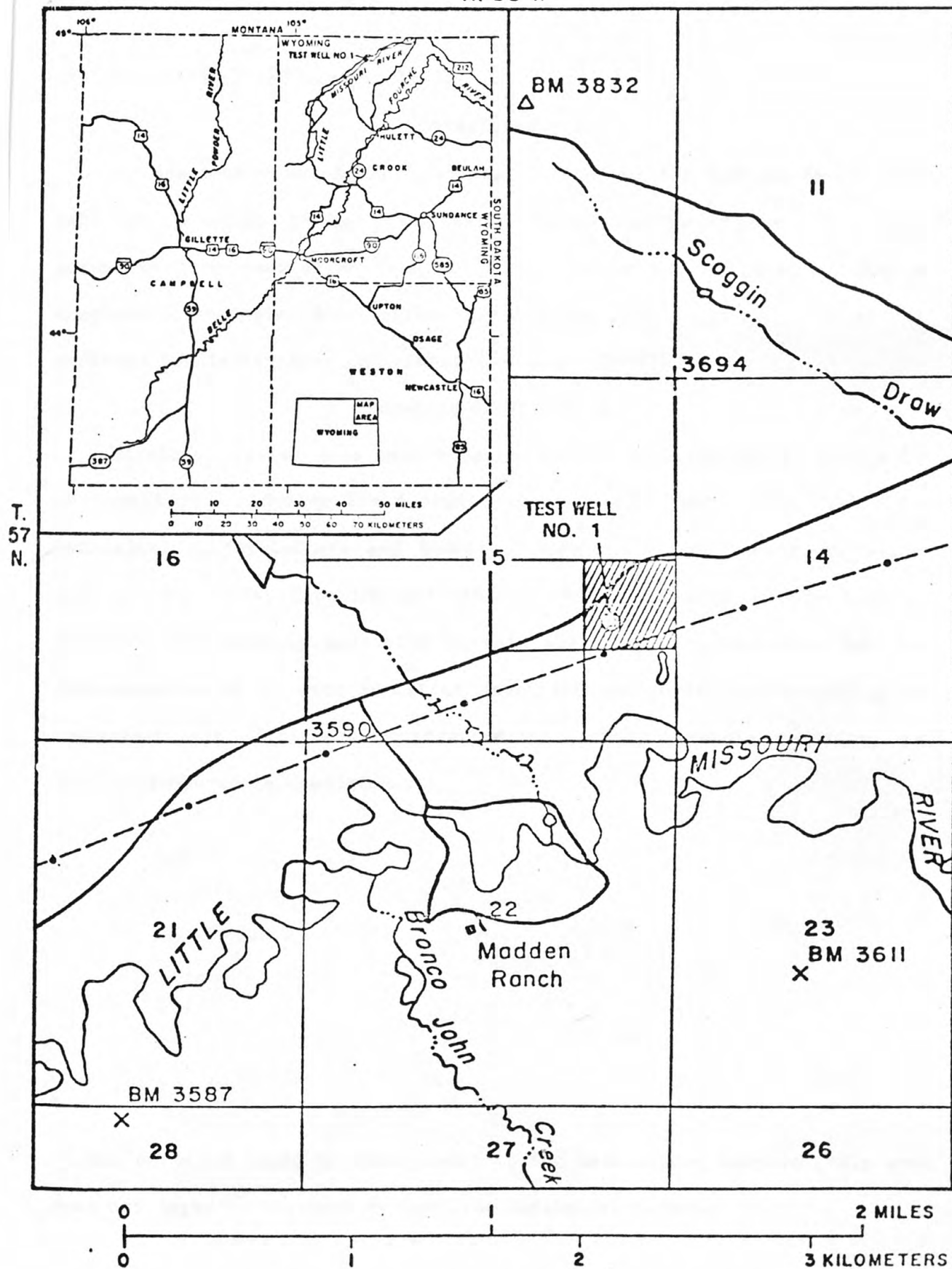
Figure 1.--Location of drilling site for Madison Group test well no. 1. (modified from Blankennagel and others, 1977)
