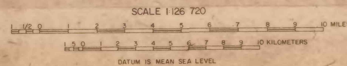
STRUCTURE CONTOUR MAP DRAWN ON BASE OF HARMON BED OR SECOND HARMON SPLIT (TONGUE RIVER MEMBER OF FORT UNION FORMATION) BOWMAN-GASCOYNE AREA ADAMS, BILLINGS, BOWMAN, GOLDEN VALLEY, AND SLOPE COUNTIES, NORTH DAKOTA
