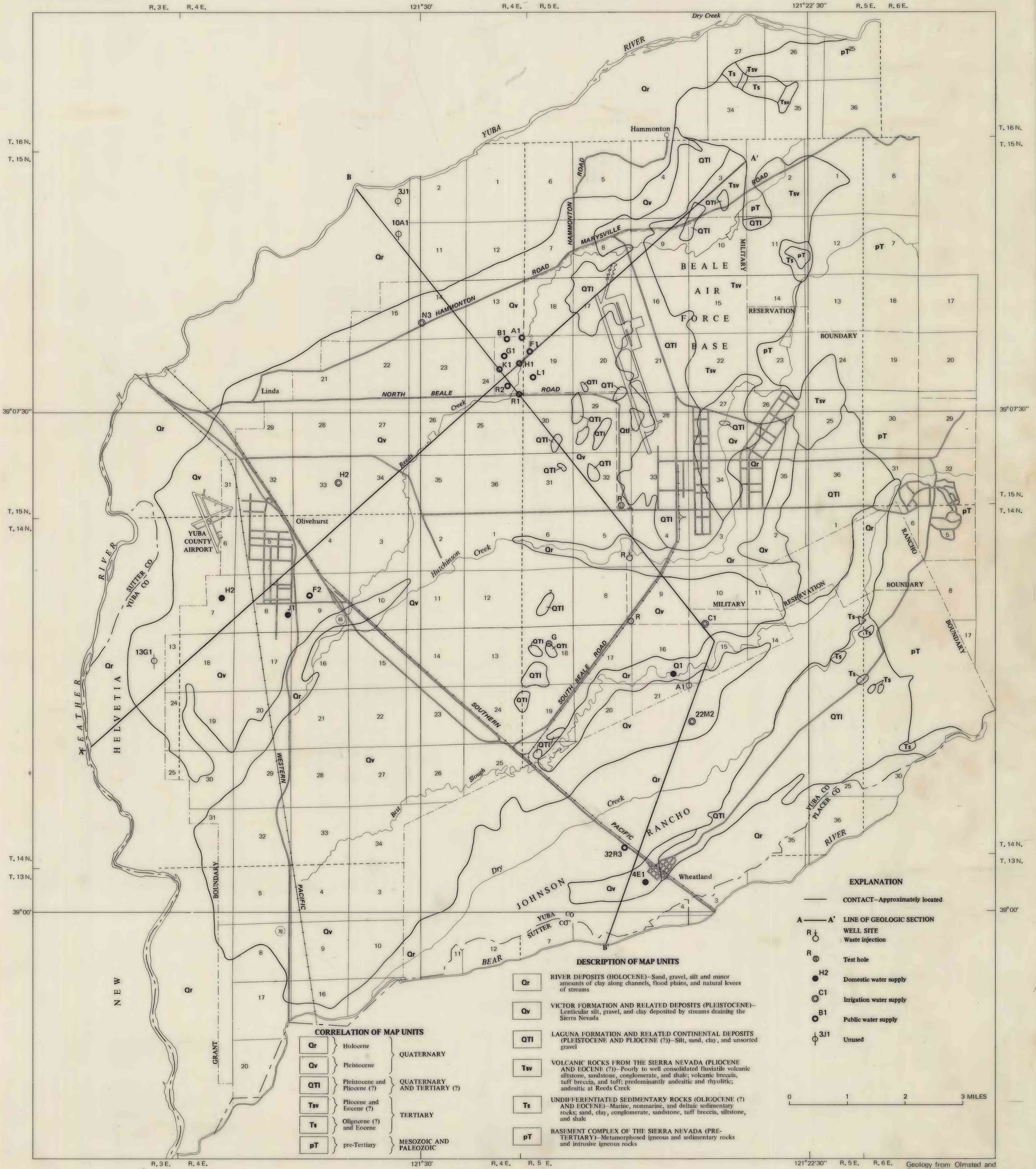
GEOLOGIC MAP OF BEALE AIR FORCE BASE AND VICINITY, CALIFORNIA
