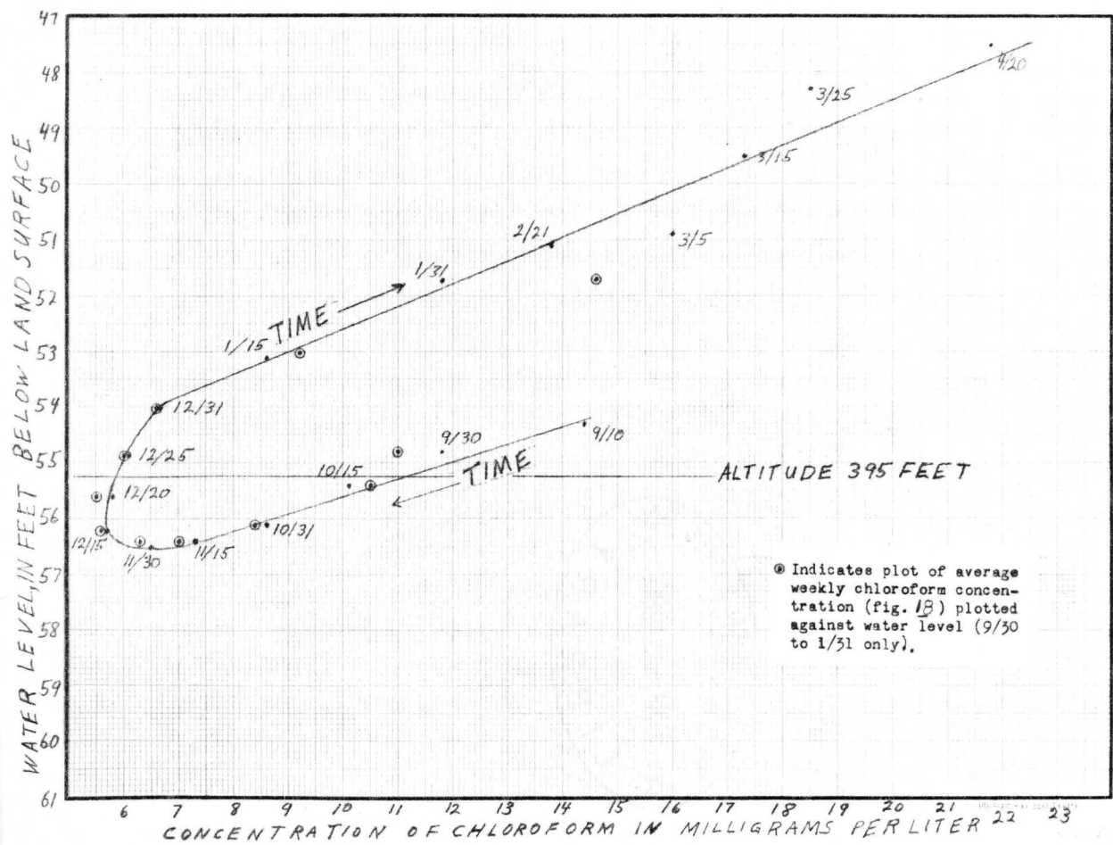
Figure 20...Chloroform concentration in water from duPont well 22 as a function of water level in a nearby observation well.
