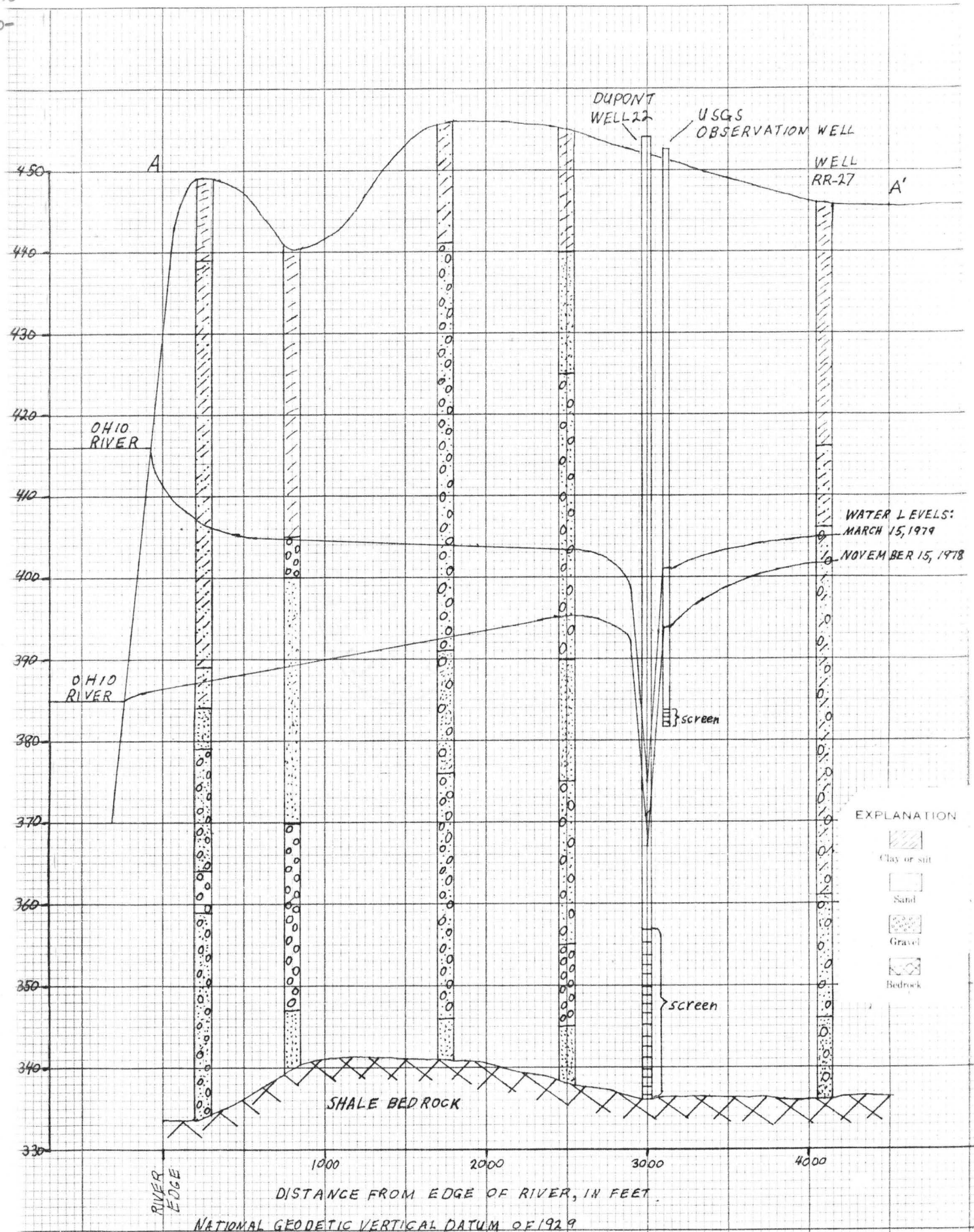
Geology modified from Price, 1964, western part of section H-H' Figure 3... Geologic section A-A' showing types of sediments in the alluvium and water level changes. Location of section shown in figure 1.
