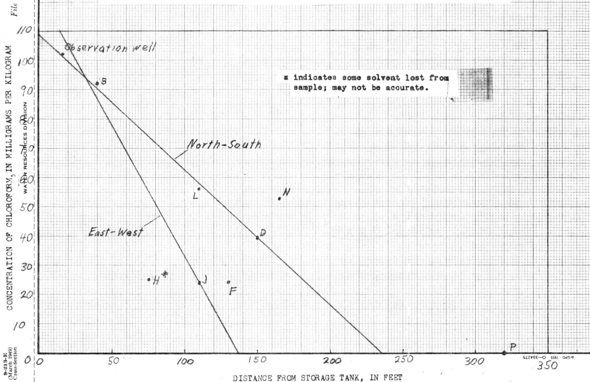
Figure 7...Concentration of chloroform in soil samples from 399-foot altitude compared to distance from northernmost small chloroform storage tank.
