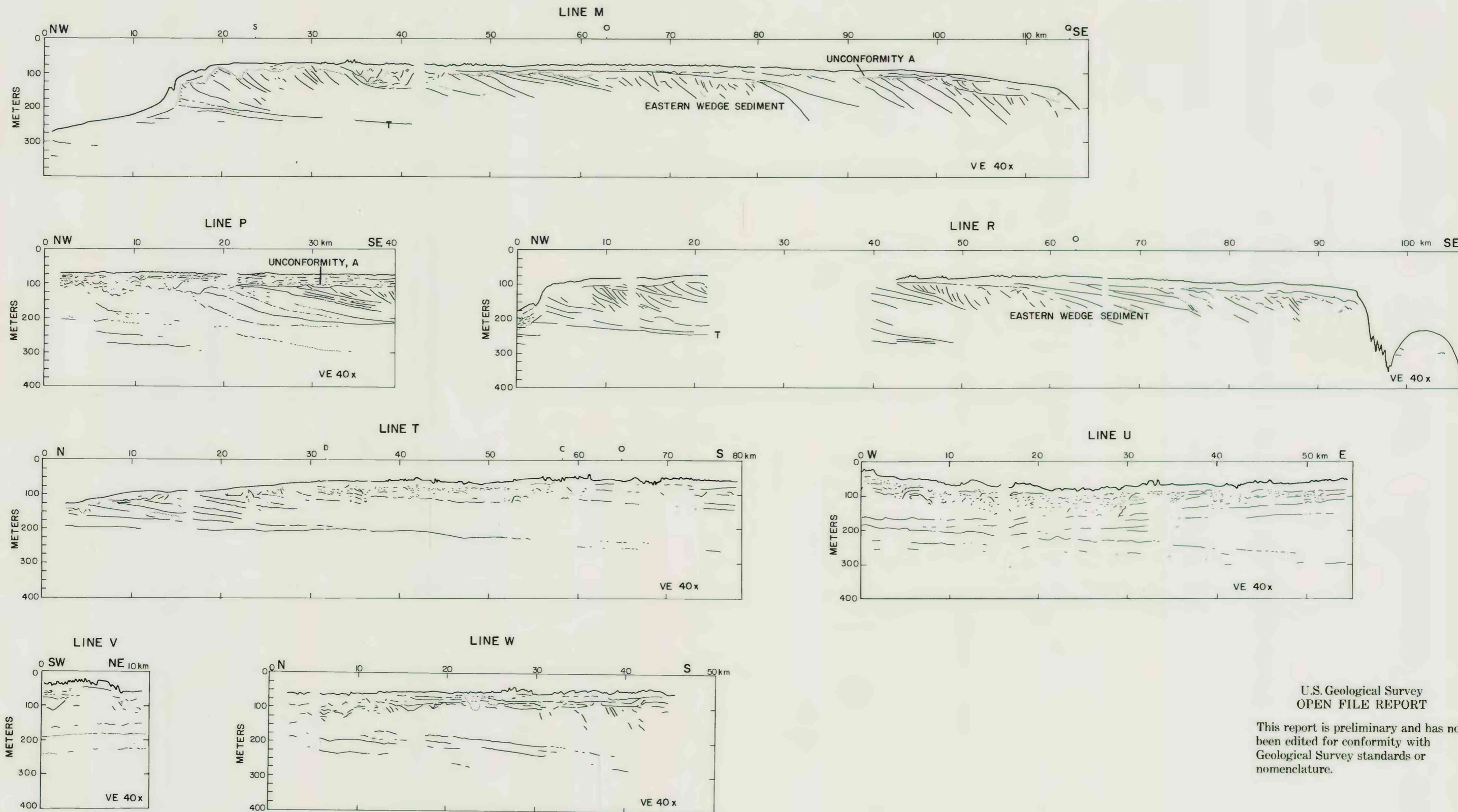
PLATE 5-3. LINE DRAWINGS OF SEISMIC-REFLECTION PROFILE LINES M, P, R, T, U, V, AND W, SHOWING SHALLOW STRUCTURE OF GEORGES BANK. REFLECTORS INFERRED TO BE OF TERTIARY AGE ARE IDENTIFIED WITH A T. THE LOCATIONS OF INTERSECTIONS WITH OTHER SEISMIC LINES IN THIS SURVEY ARE INDICATED BY THE LINE LETTER DESIGNATIONS ACROSS THE TOP OF EACH SECTION. DEPTHS ARE IN METERS BELOW SEA LEVEL.
