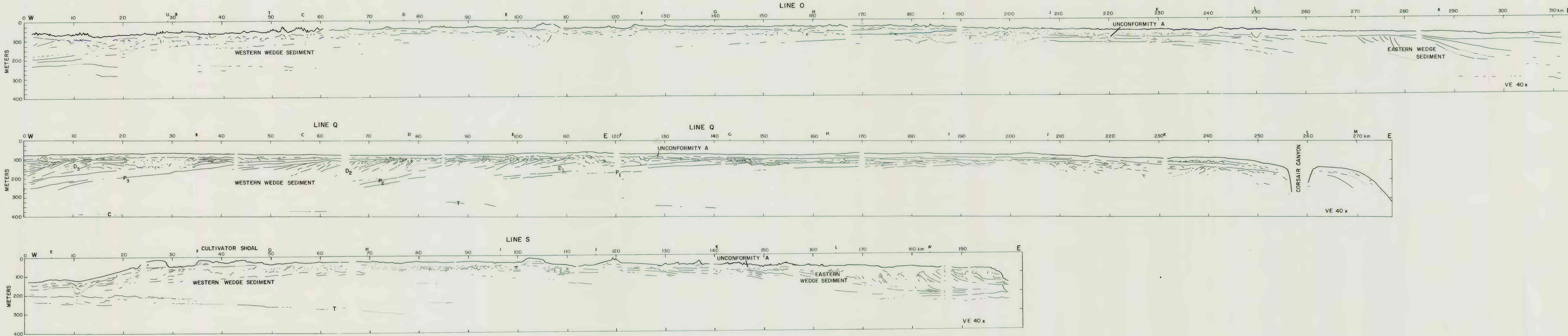
PLATE 5-4. LINE DRAWINGS OF SEISMIC-REFLECTION PROFILE LINES O, Q, AND S, SHOWING SHALLOW STRUCTURE OF GEORGES BANK. REFLECTORS P 1 , P 2 , AND P 3 ARE INFERRED TO BE EROSION SURFACES (UNCONFORMITIES); AREAS D 1 , D 2 , AND D 3 REPRESENT PERIODS OF DEPOSITION. REFLECTORS INFERRED TO BE OF TERTIARY AGE ARE IDENTIFIED WITH A T; REFLECTORS INFERRED TO BE OF CRETACEOUS AGE ARE IDENTIFIED WITH A C. THE LOCATIONS OF INTERSECTIONS WITH OTHER SEISMIC LINES IN THIS SURVEY ARE INDICATED BY THE LINE LETTER DESIGNATIONS ACROSS THE TOP OF EACH SECTION. DEPIHS ARE IN METERS BELOW SEA LEVEL.
