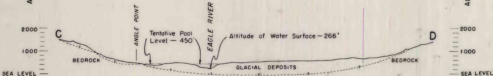
GEOLOGIC CROSS SECTION EAGLE RIVER VALLEY, ALASKA DAM SITE AREA NO. 2
