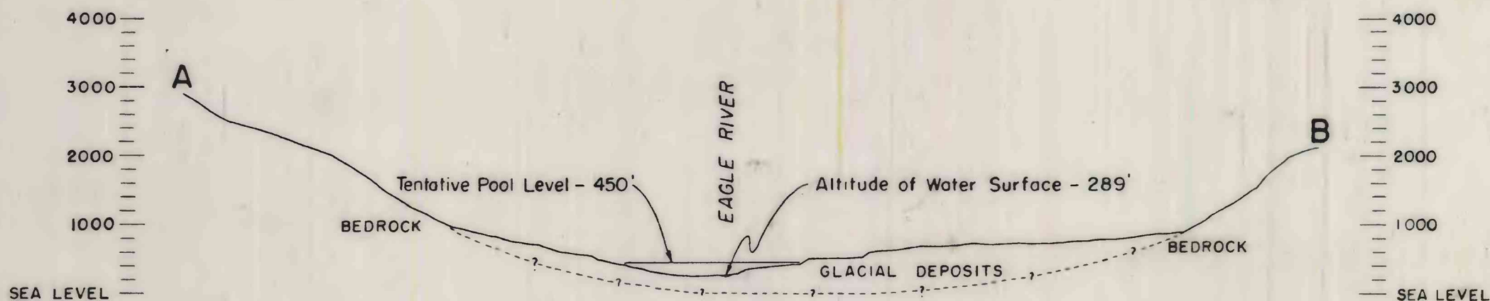
GEOLOGIC CROSS SECTION EAGLE RIVER VALLEY, ALASKA DAM SITE AREA NO. 1
