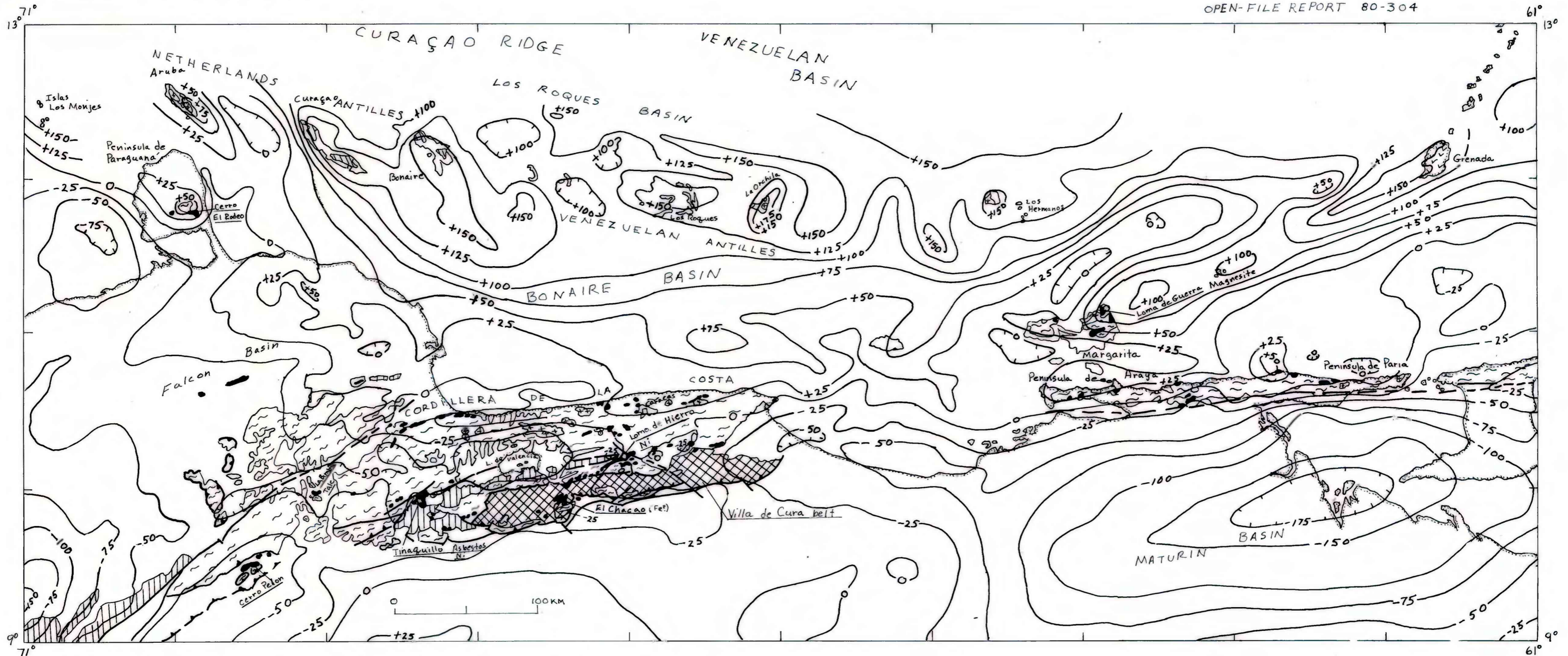
Figure 23. Simplified geologic map and Bouguer anomaly map of northern Venezuela and vicinity. Gravity data modified from Bonini and others (1977). Contour interval 25 mgal. Ultramafic and gabbroic masses in shaded pattern. Metamorphic rocks (Mesozoic) in lazy-s pattern. Vertical rule indicates Paleozoic and Precambrian igneous and metamorphic complex. Cross-hatch indicates rocks of blueschist facies. Plus pattern indicates intermediate to silicic plutons. Diagonal rule indicates mafic volcanic rocks, relatively unmetamorphosed. Vee-pattern indicates younger volcanic rocks of Lesser Antilles.
