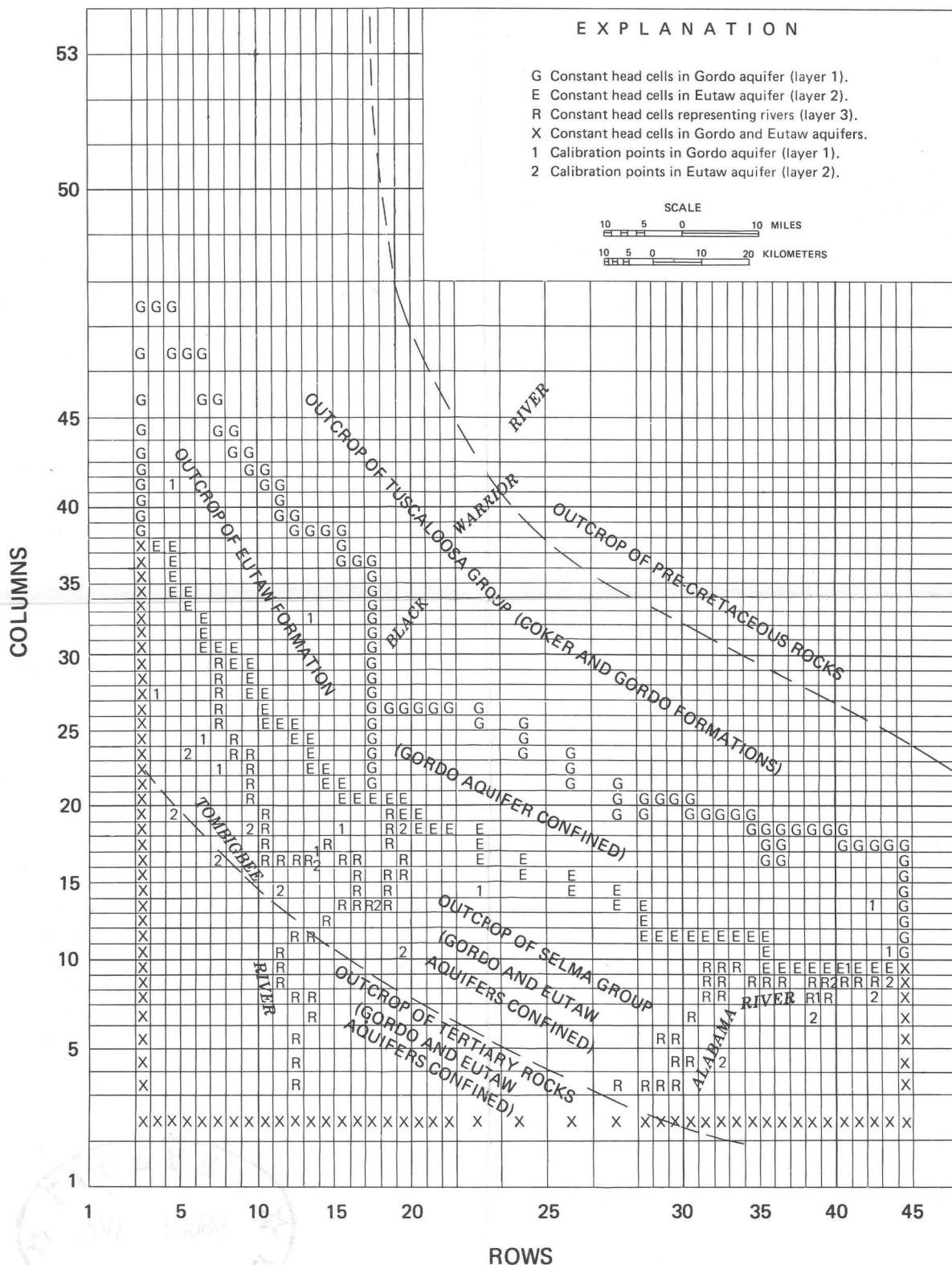
Figure 10.--Finite difference grid showing constant head boundary cells and calibration points.
