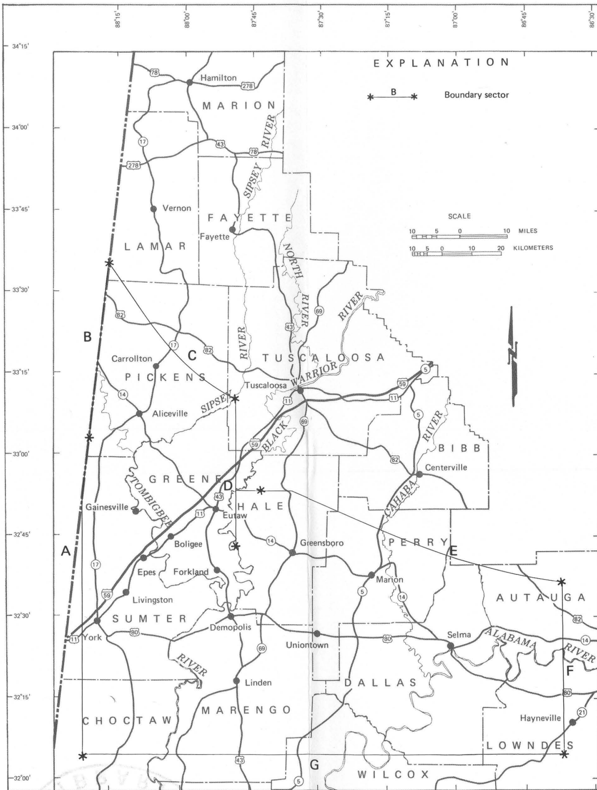
Figure 14.--Boundary sectors in the Gordo aquifer for which net flow to constant head cells is computed.
