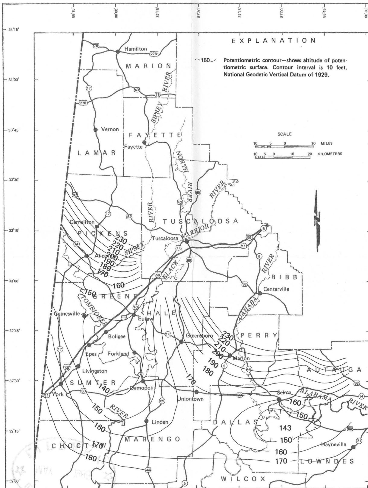
Figure 16.--Computed potentiometric surface in the Gordo aquifer, model simulation I.
