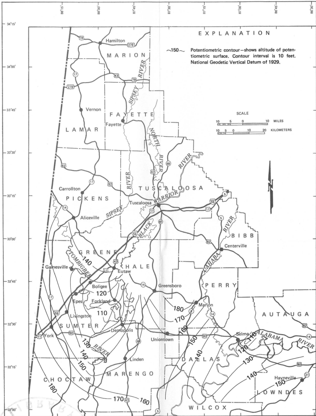
Figure 17.--Computed potentiometric surface in the Eutaw aquifer, model simulation I.
