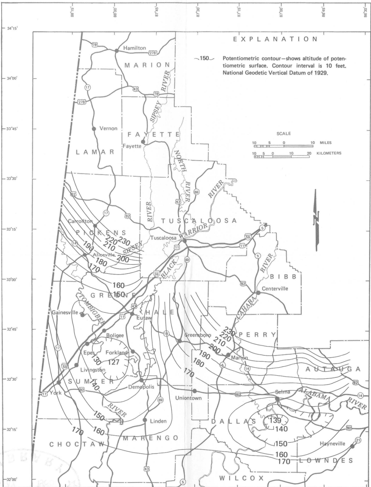
Figure 18.--Computed potentiometric surface in the Gordo aquifer, model simulation II.
