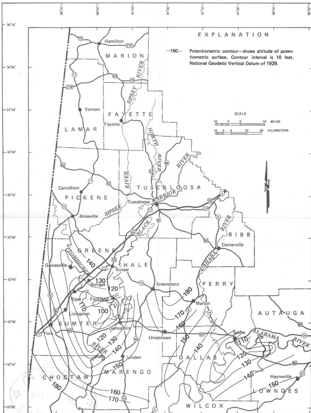
Figure 19.--Computed potentiometric surface in the Eutaw aquifer, model simulation II.
