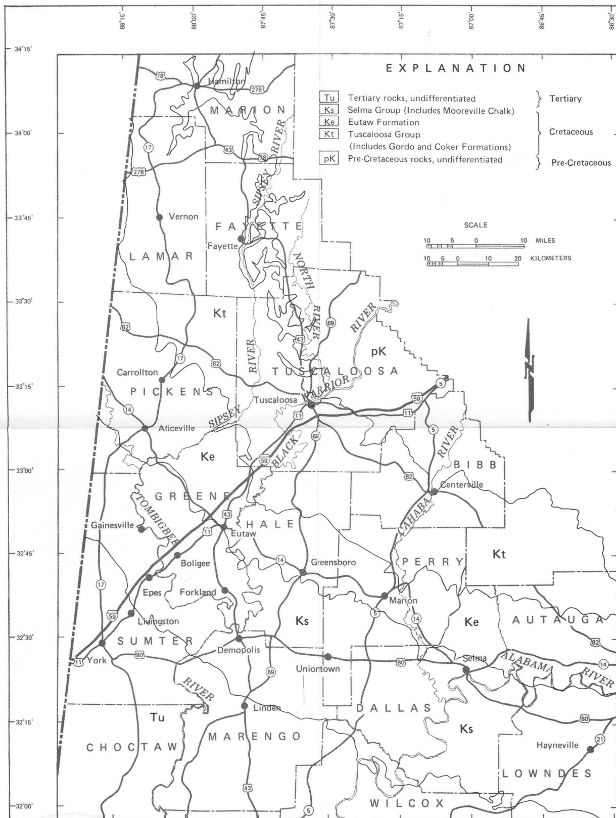
Figure 2.--Generalized geologic map of the study area.
