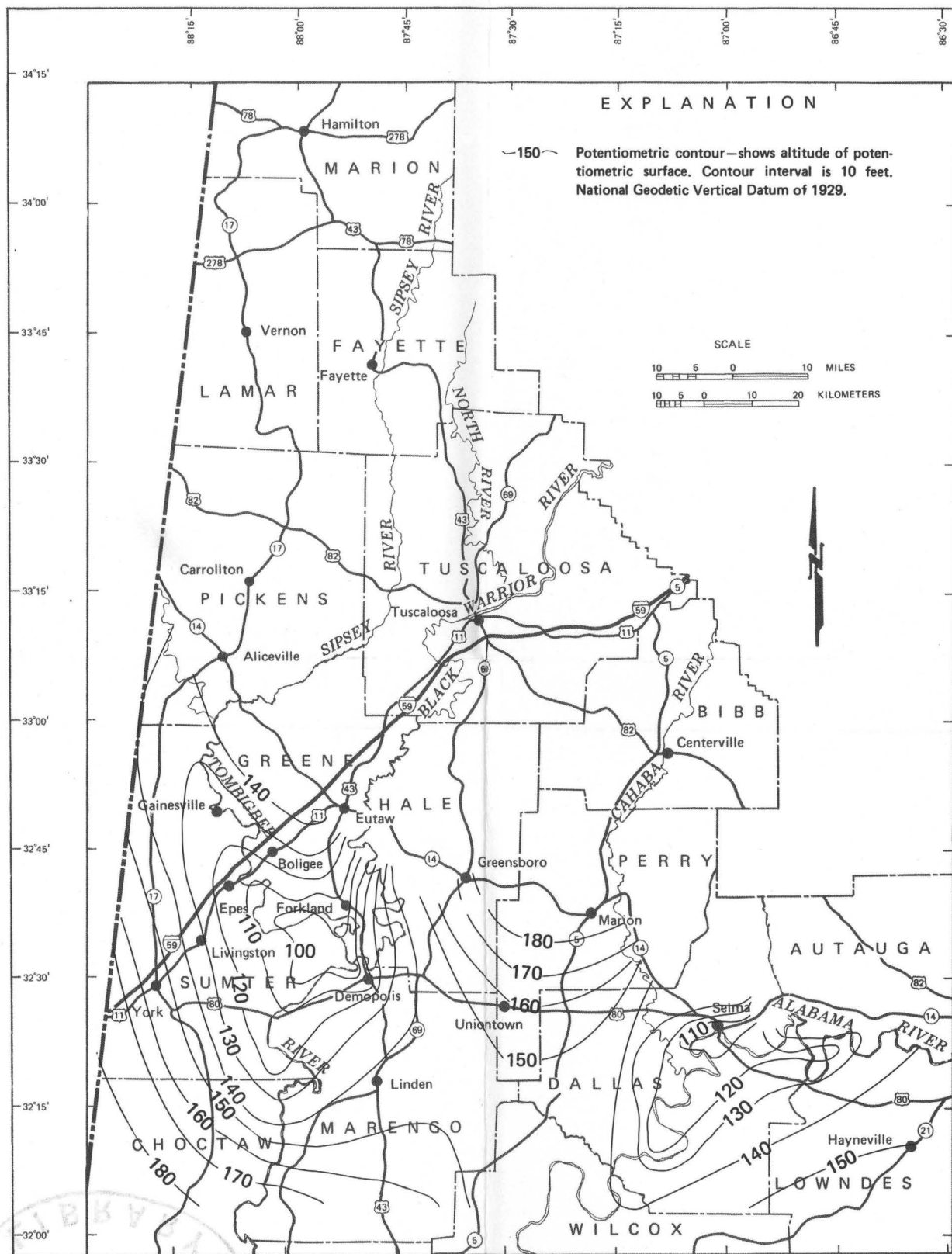
Figure 21.—Computed potentiometric surface in the Eutaw aquifer, model simulation III.
