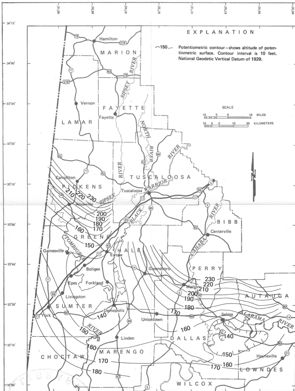
Figure 22.--Computed potentiometric surface in the Gordo aquifer, model simulation IV.
