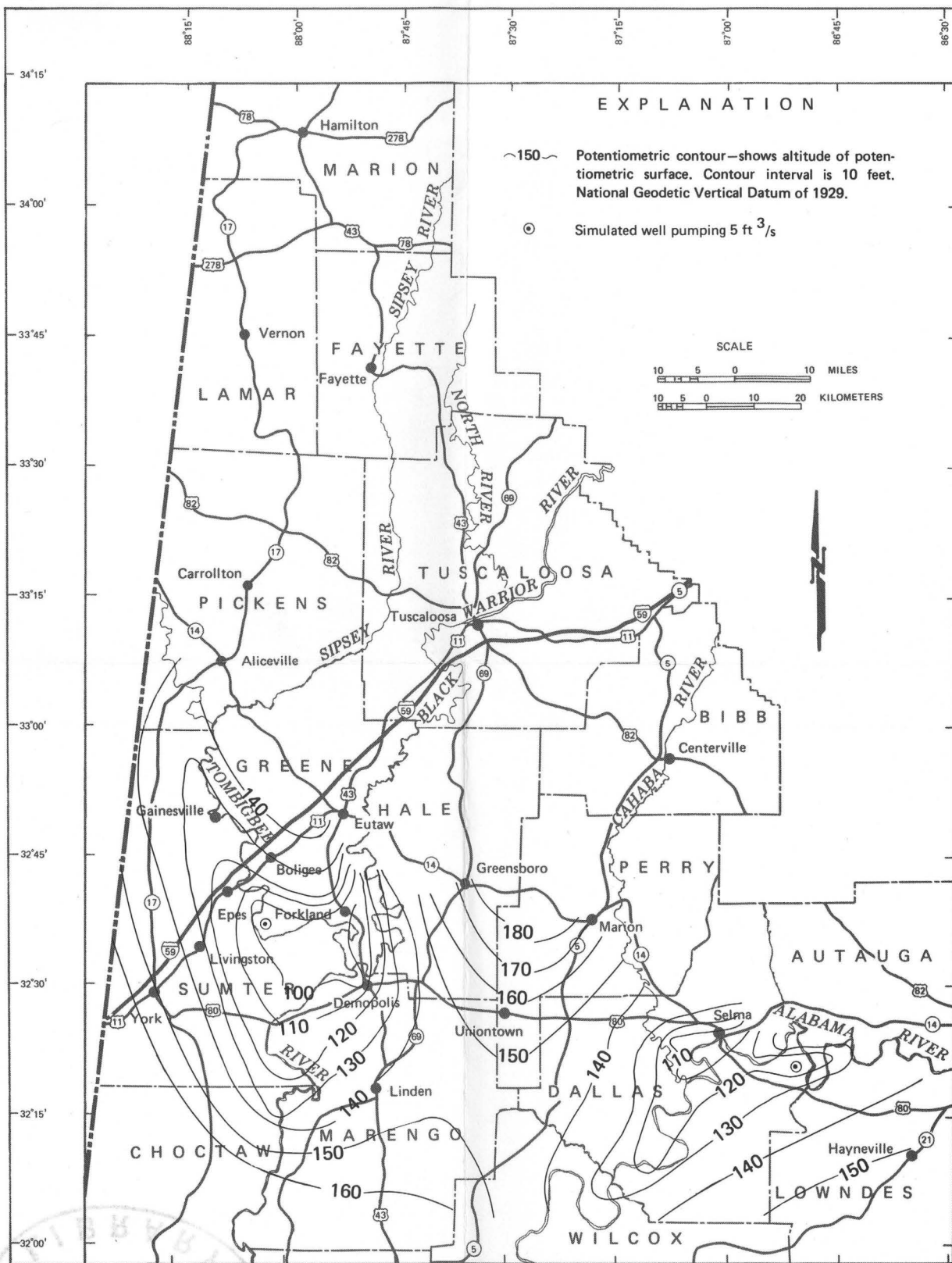
Figure 25.--Computed potentiometric surface in the Eutaw aquifer and locations of additional simulated pumping wells, model simulation V.
