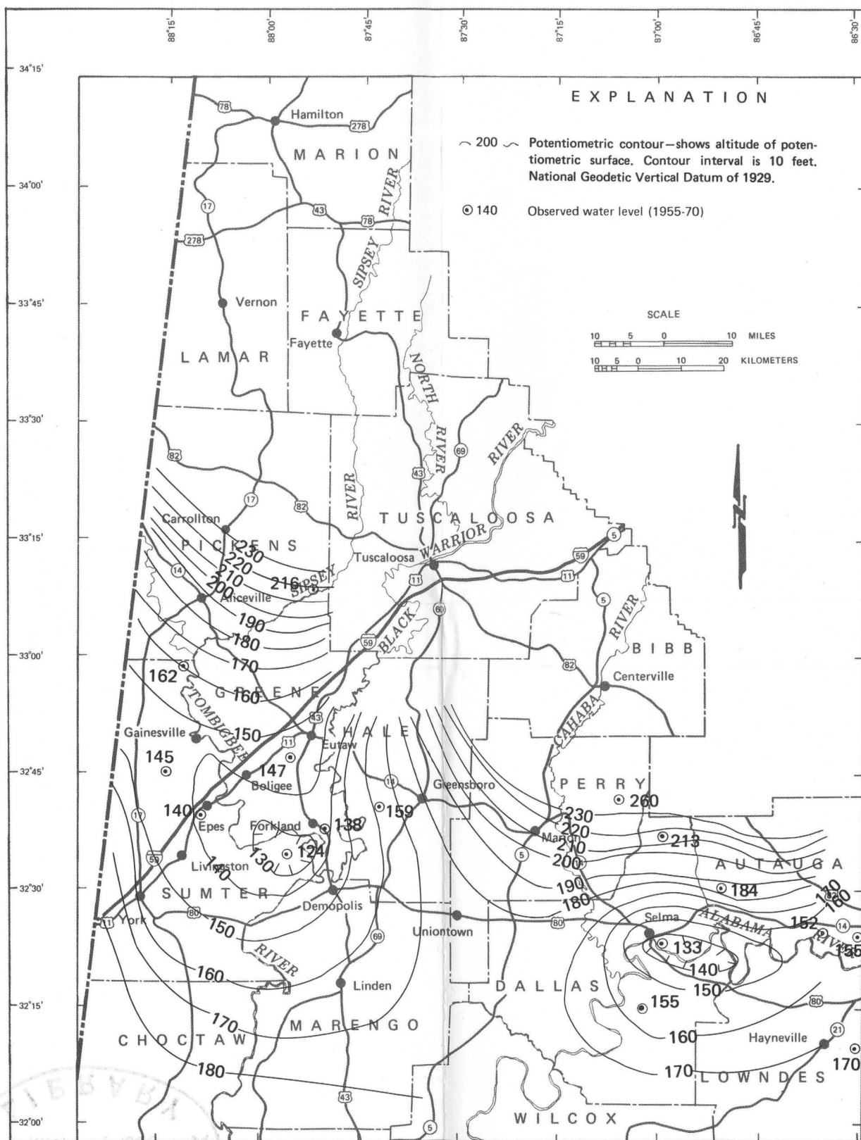
Figure 6.--Potentiometric surface in the Gordo aquifer 1955-70.
