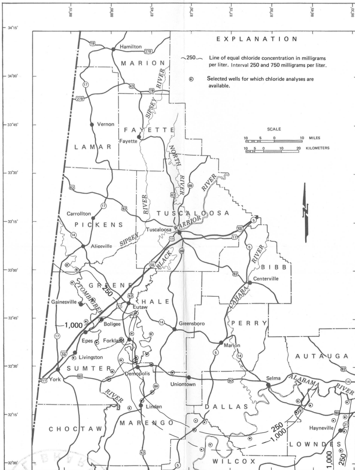
Figure 8.--Chloride concentration in water of the Eutaw aquifer.
