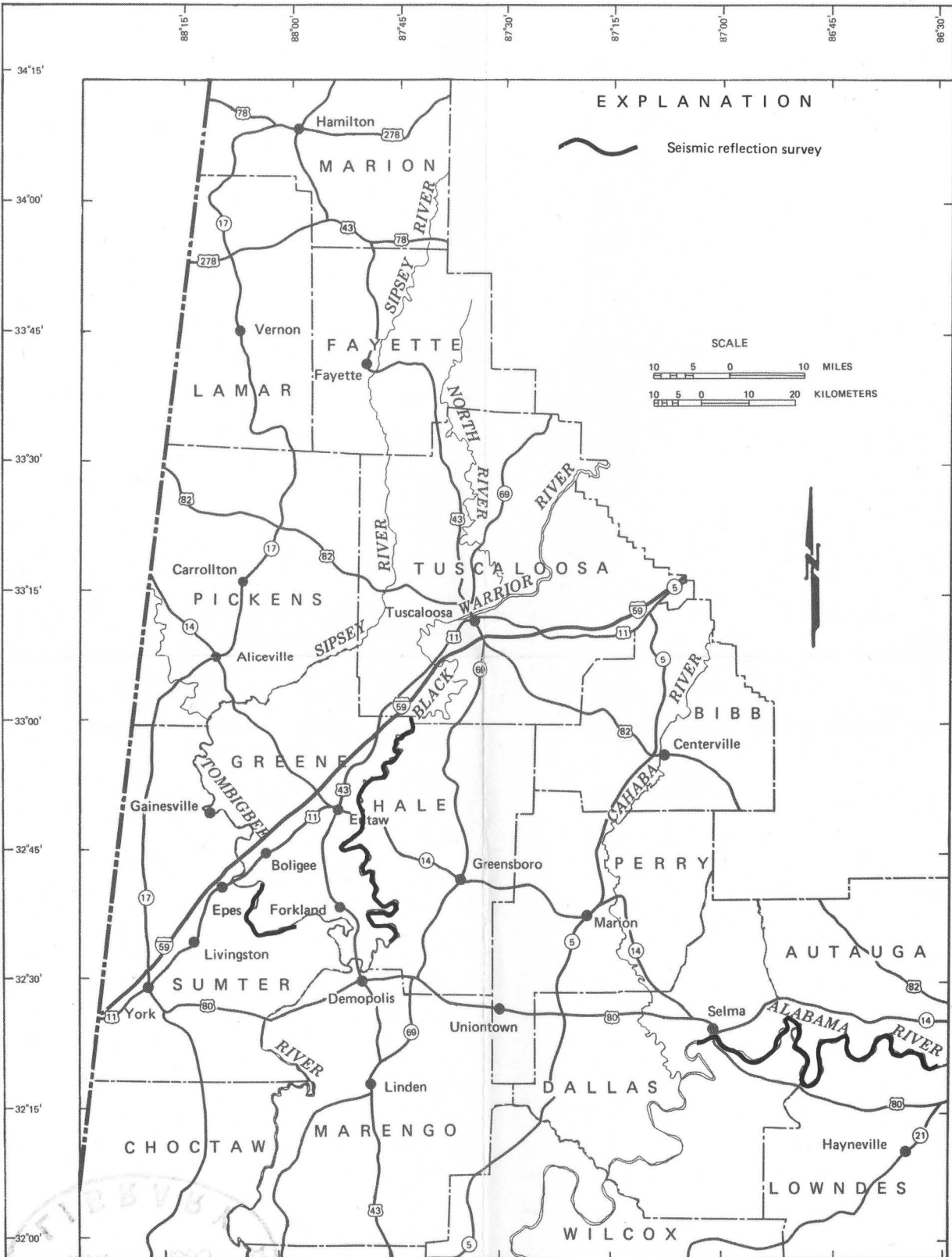
Figure 9.--Reaches in the Alabama, Black Warrior, and Tombigbee Rivers where continuous reflection seismic surveys were conducted.
