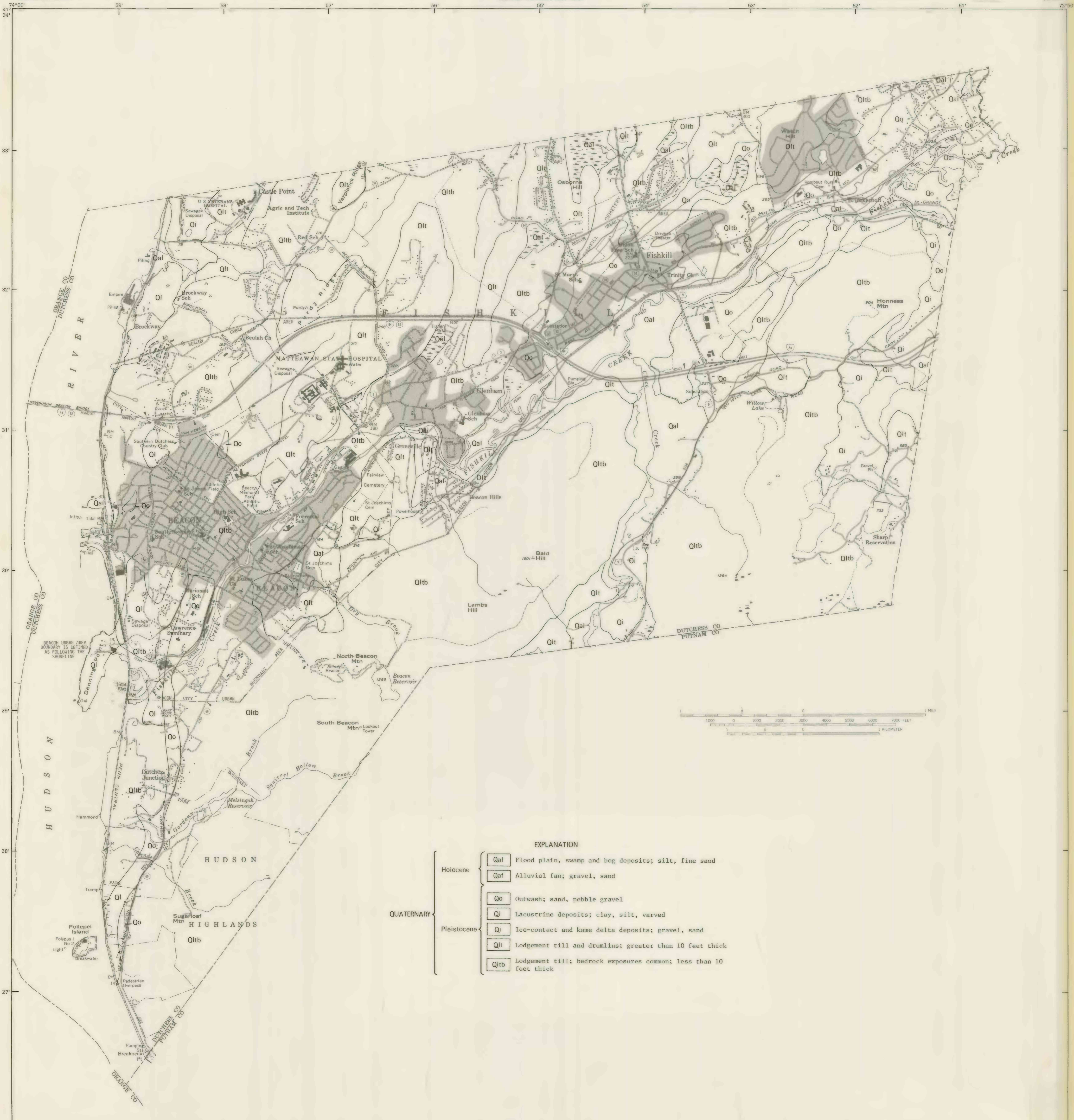
SURFICIAL GEOLOGY OF THE FISHKILL-BEACON AREA
