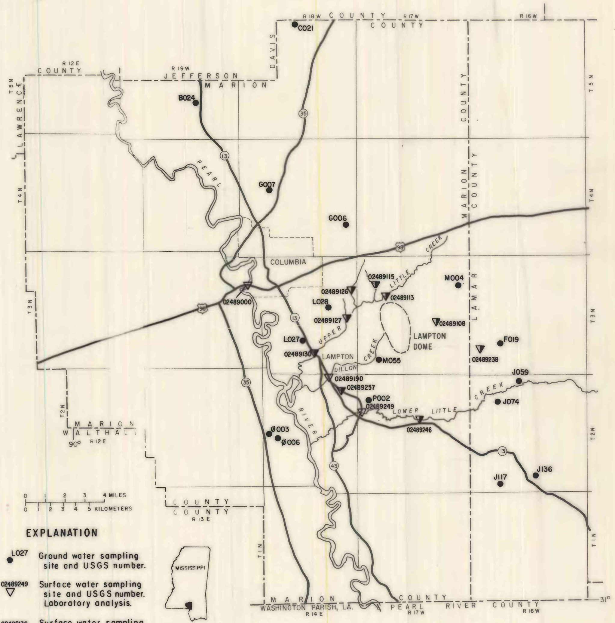
Figure 3.--Location of surface-water and ground-water sampling sites in Marion and Lamar Counties, Mississippi.
