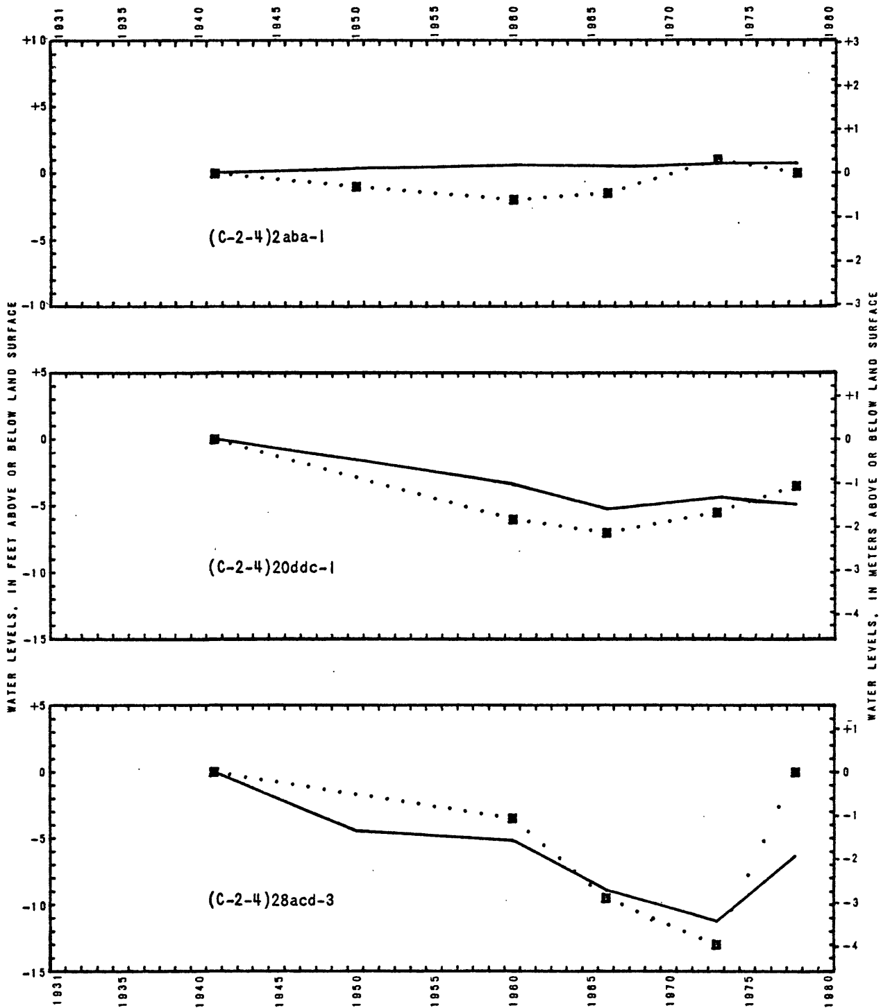
Figure 3.--Hydrographs of selected wells showing observed and computed water-level changes. Dotted line is hydrograph based on actual measurements shown by aquares; solid line is computed hydrograph.
