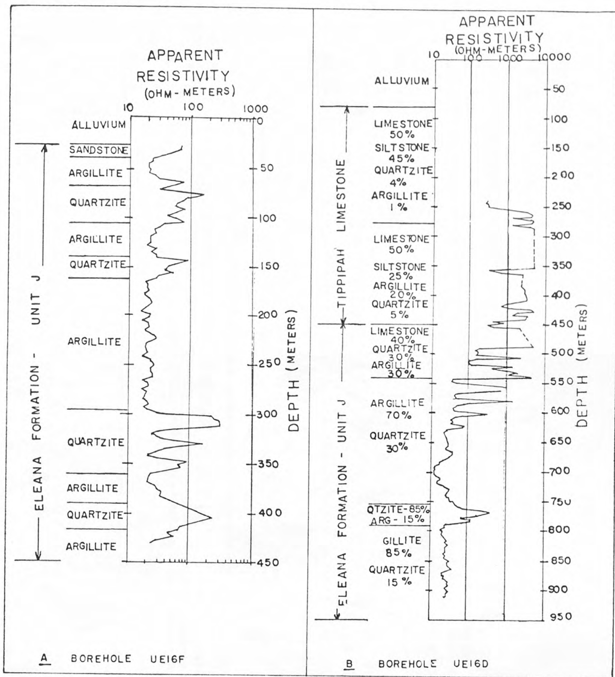
Figure 2.--Resistivity variations as a function of rock type determined from boreholes; A , UE16F; and B , UE16D located as shown in figure 1.
