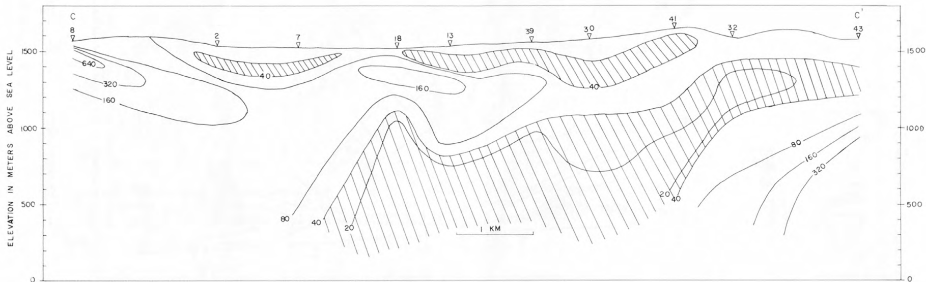
Figure 5.--Geoelectric cross-section C-C' (fig. 1) compiled from interpreted resistivity sounding data. Contours increase in geometric progression from a value of 20 ohm-meters. Patterned areas are those intervals considered to be composed primarily of argillaceous argillite of the Eleana Formation. Vertical exaggeration is 2X.
