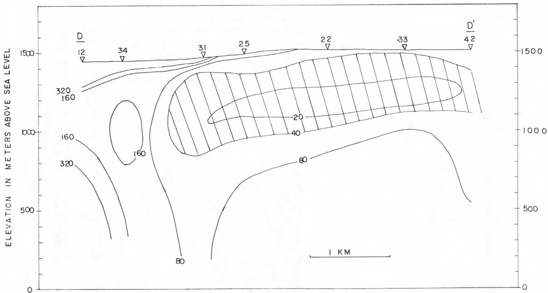
Figure 6.--Geoelectric cross-section D-D' (fig. 1) compiled from interpreted resistivity sounding data. Contours increase in geometric progression from a value of 20 ohm-meters. Patterned areas are those intervals considered to be composed primarily of argillaceous argillite of the Eleana Formation. Vertical exaggeration is 2X.
