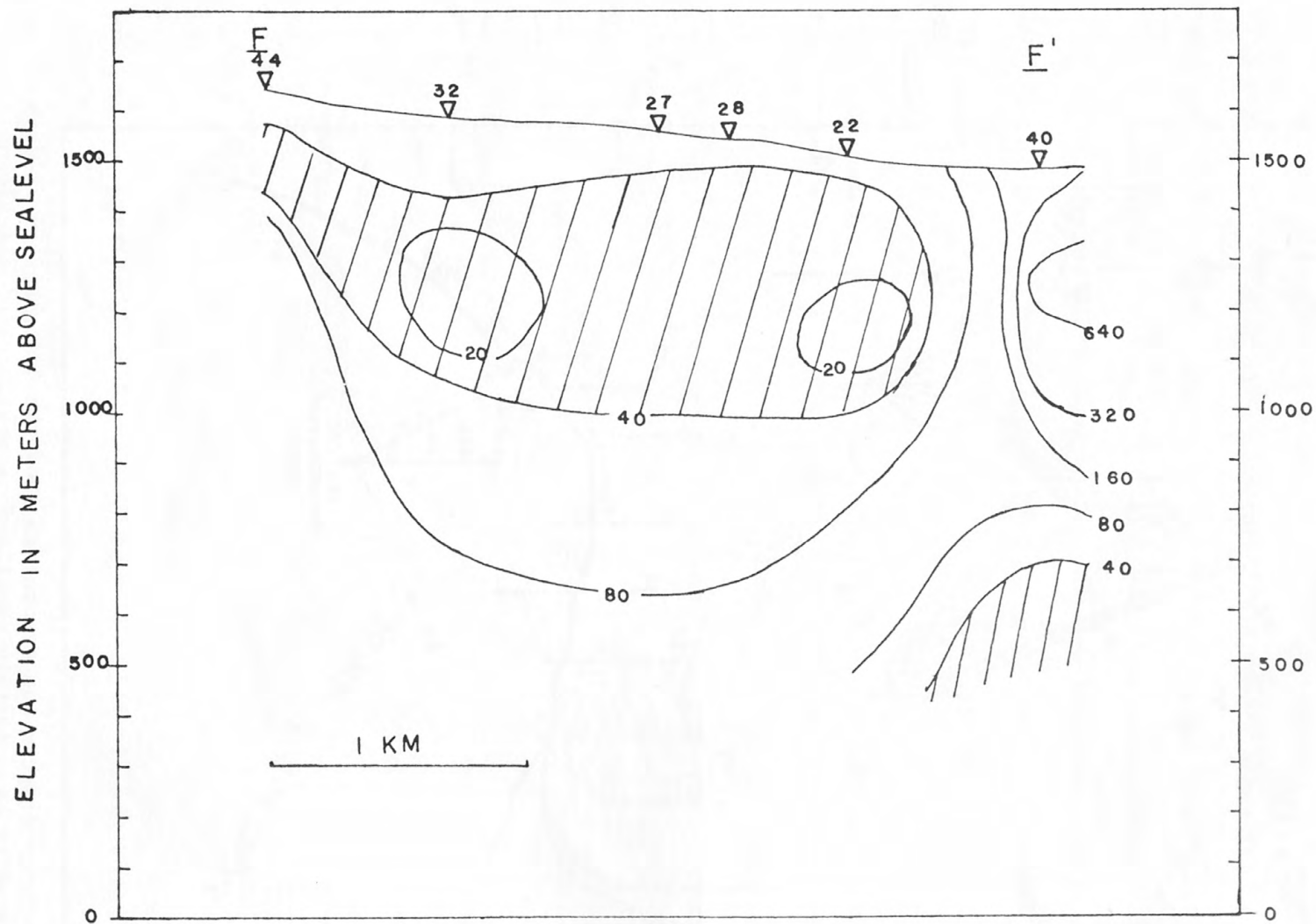
Figure 8.--Geoelectric cross-section \underline{F-F'} (fig. 1) compiled from interpreted resistivity sounding data. Contours increase in geometric progression from a value of 20 ohm-meters. Patterned areas are those intervals considered to be composed primarily of argillaceous argillite of the Eleana Formation. Vertical exaggeration is 2X.
