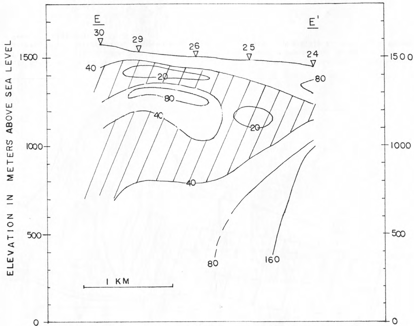
Figure 7.--Geoelectric cross-section E-E (fig. 1) compiled from interpreted resistivity sounding data. Contours increase in geometric progression from a value of 20 ohm-meters. Dashed contours indicate inferred values of resistivity. Patterned areas are those intervals considered to be composed primarily of argillaceous argillite of the Eleana Formation. Vertical exaggeration is 2X.
