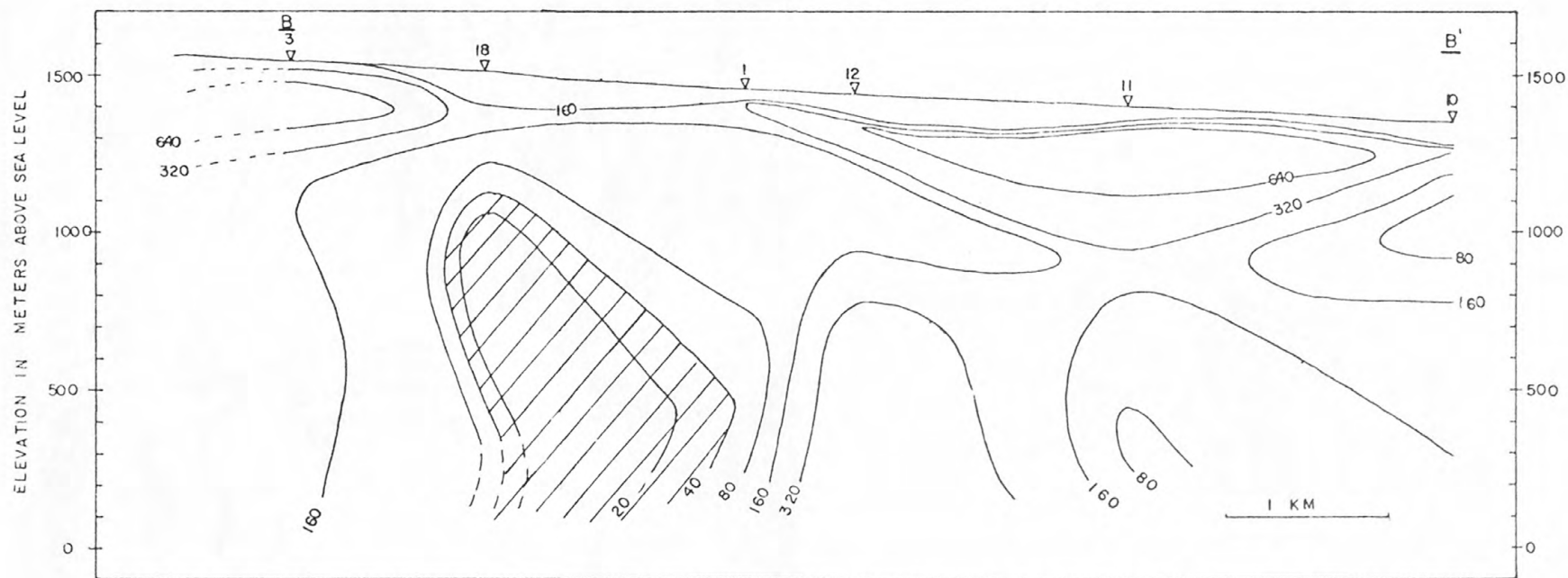
Figure 4.--Geoelectric cross-section B-B' (fig. 1) compiled from interpreted resistivity sounding data. Contours increase from a value of 20 ohm-meters. Dashed contours indicate inferred values of resistivity. Patterned areas are those intervals considered to be composed primarily of argillaceous argillite of the Eleana Formation. Vertical exaggeration is 2X.
