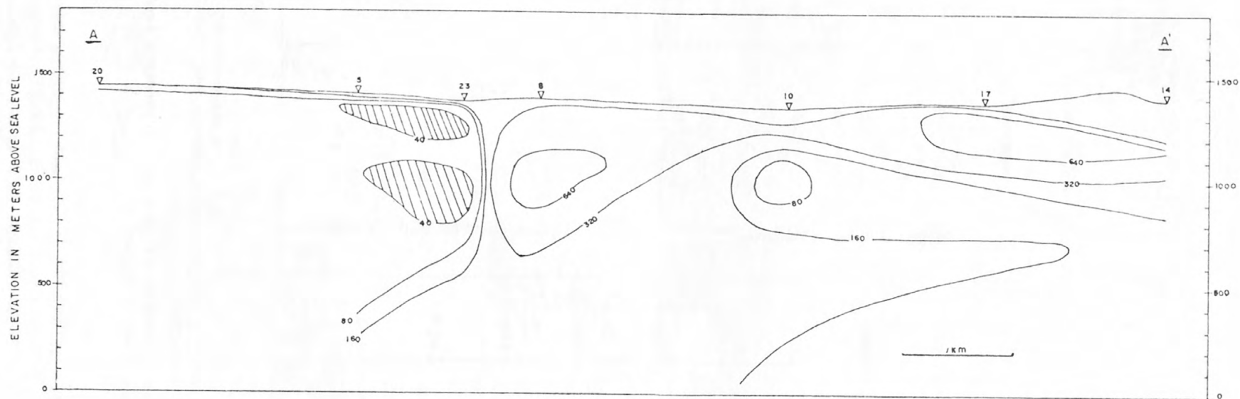
Figure 3.--Geoelectric cross-section A-A' (fig. 1) compiled from interpreted resistivity sounding data. Contours increase in geometric progression from a value of 20 ohm-meters. Patterned areas are those intervals considered to be composed primarily of argillaceous argillite of the Eleana Formation. Vertical exaggeration is 2X.
