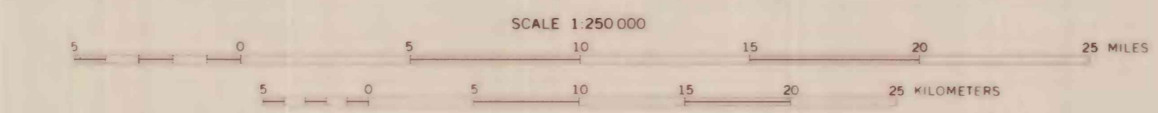
LEASABLE MINERAL AND WATERPOWER LAND CLASSIFICATION MAP OF THE DUBOIS QUADRANGLE, IDAHO, MONTANA LANDS WITHDRAWN, CLASSIFIED, AND PROSPECTIVELY VALUABLE FOR LEASABLE MINERALS; OCCURRENCES OF OTHER SELECTED MINERALS, AND LANDS WITHDRAWN OR CLASSIFIED FOR WATERPOWER AND RESERVOIR SITES Compiled by
