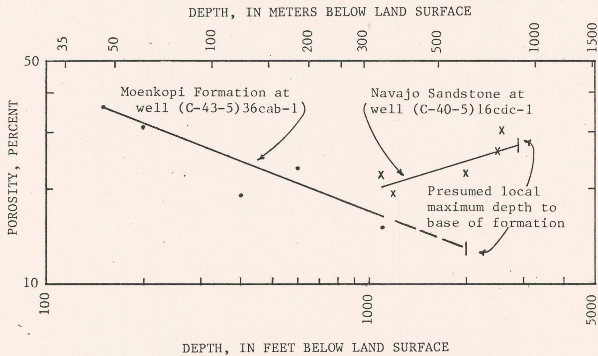
Figure 10.--Relation between porosity and depth for two aquifers in the Kanab Creek drainage basin.
