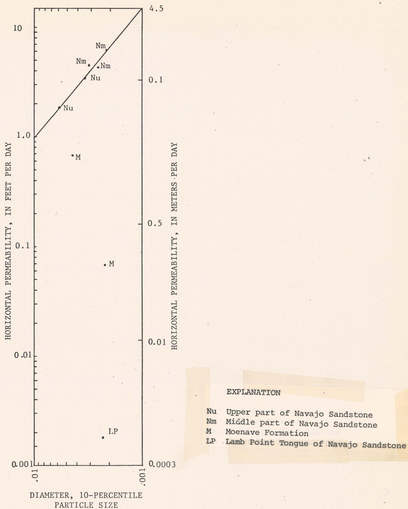
Figure 11.--Relation of horizontal permeability to the 10-percentile particle-size diameter of selected rock samples.
