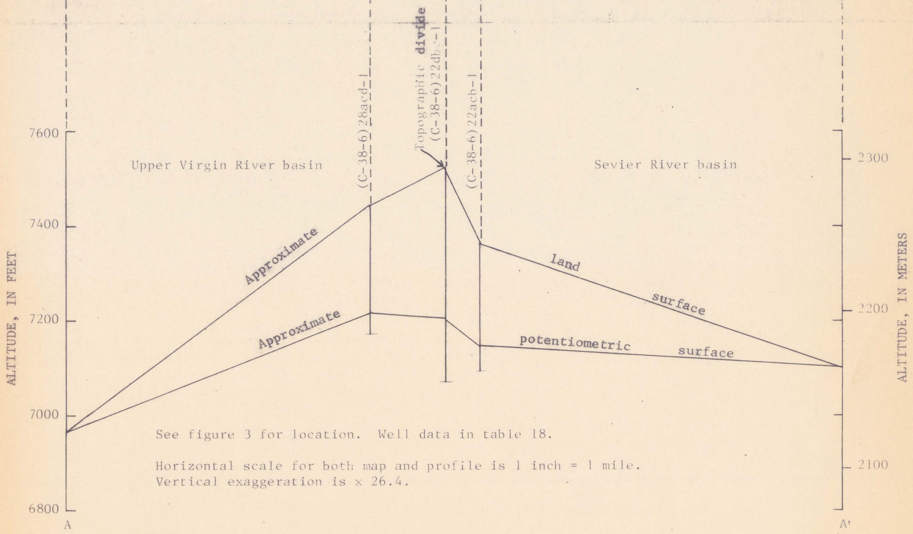
Figure 12.--Profile of the potentiometric surface at the divide between the upper Virgin River and Sevier River basins.
