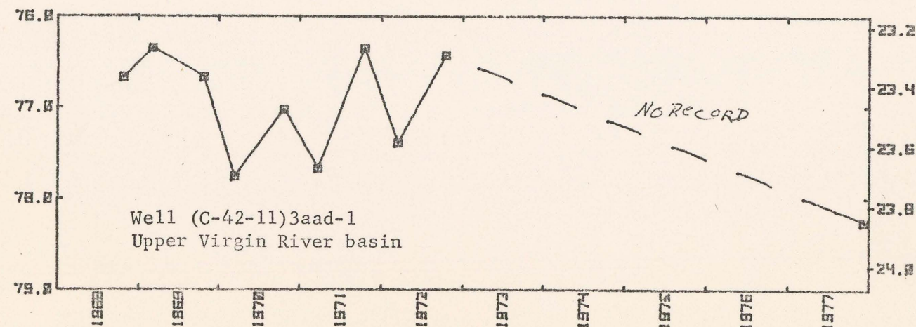
Figure 13.--Water-level fluctuations in selected wells in the study area.
