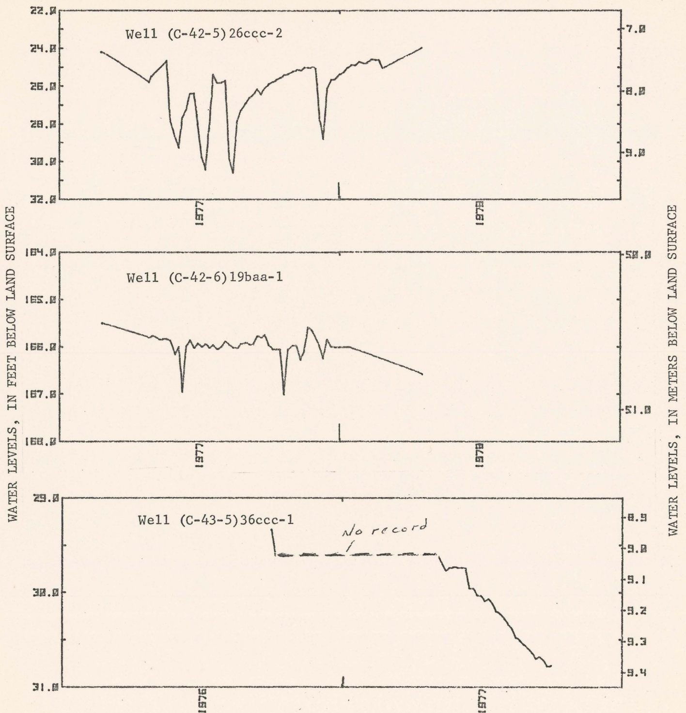
Figure 14.--Water-level fluctuations (1976-78) in selected wells in selected wells in the upper Kanab Creek basin.
