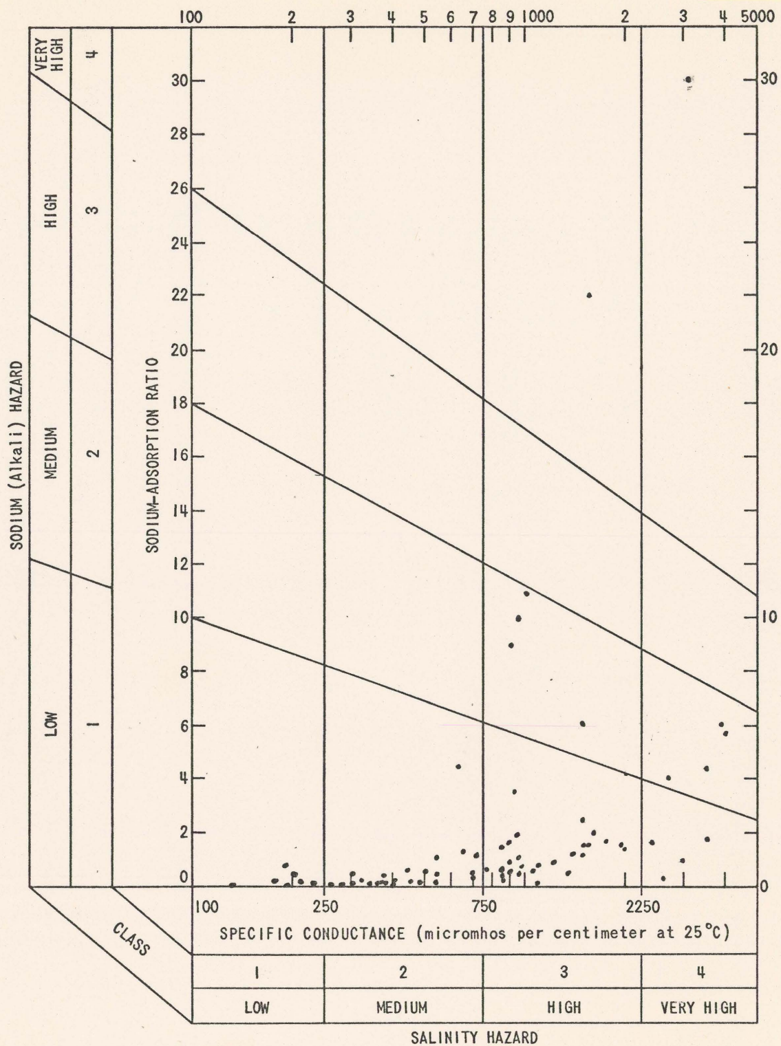
Figure 18.--Classification for irrigation of selected ground-water samples from the study area (after U.S. Salinity Laboratory Staff, 1954).
