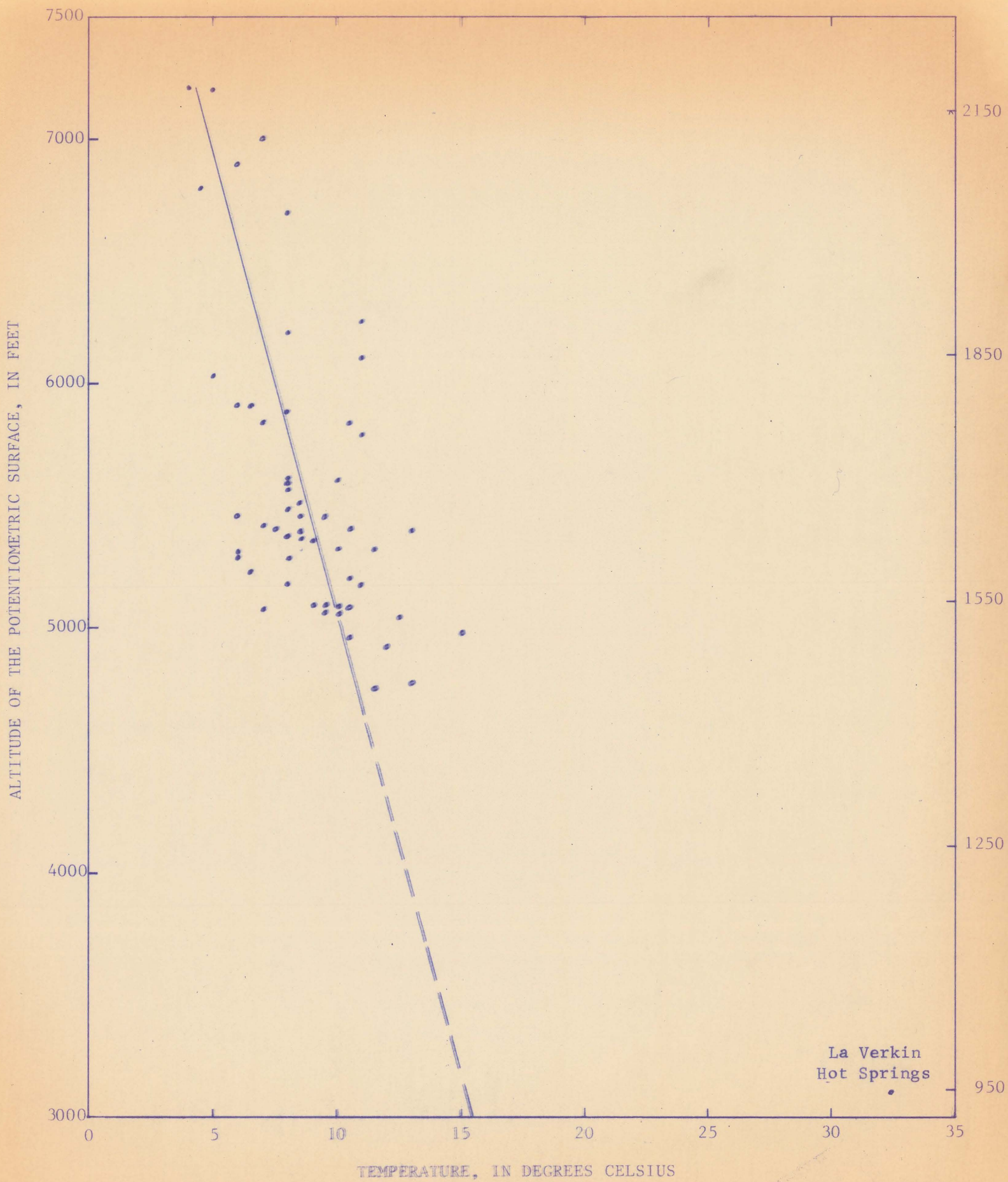
Figure 19.--Relation of ground-water temperature to the altitude of the potentiometric surface.
