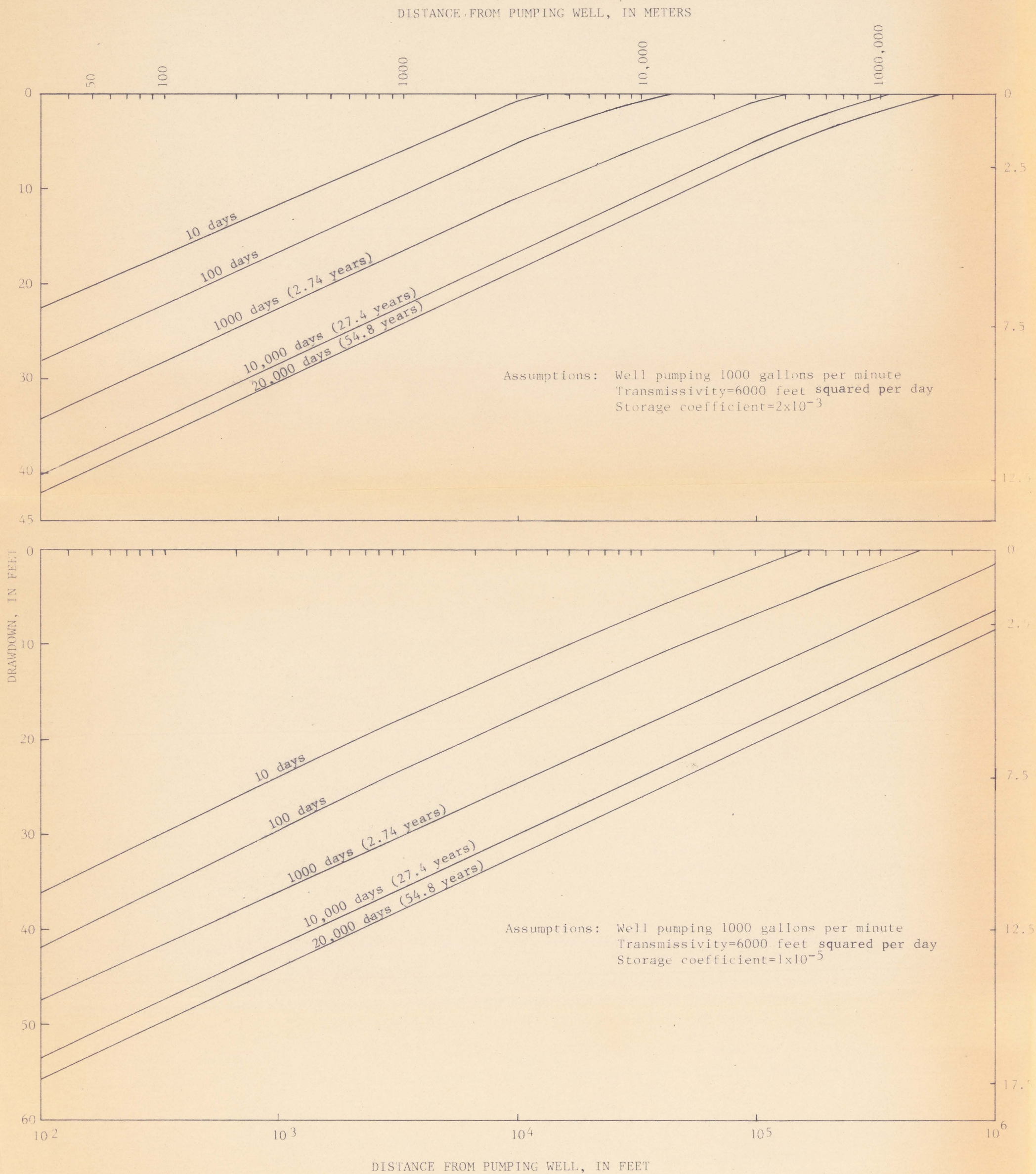
Figure 20.--Theoretical relation between drawdown and distance from a pumping well in the Navajo Sandstone for selected pumping durations.
