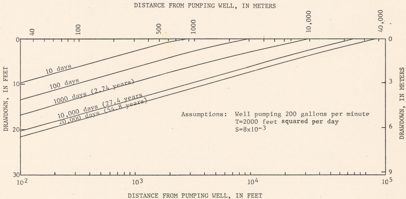
Figure 21.--Theoretical relation between drawdown and distance from a pumping well tapping mainly the Shinarump Member of the Chinle Formation for selected pumping periods.
