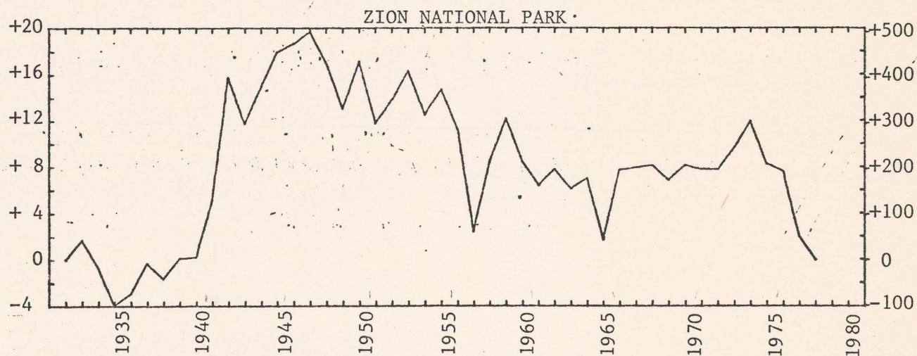
Figure 5.--Cumulative departure from average annual precipitation for the respective periods of record of climatologic stations in and near the study area.
