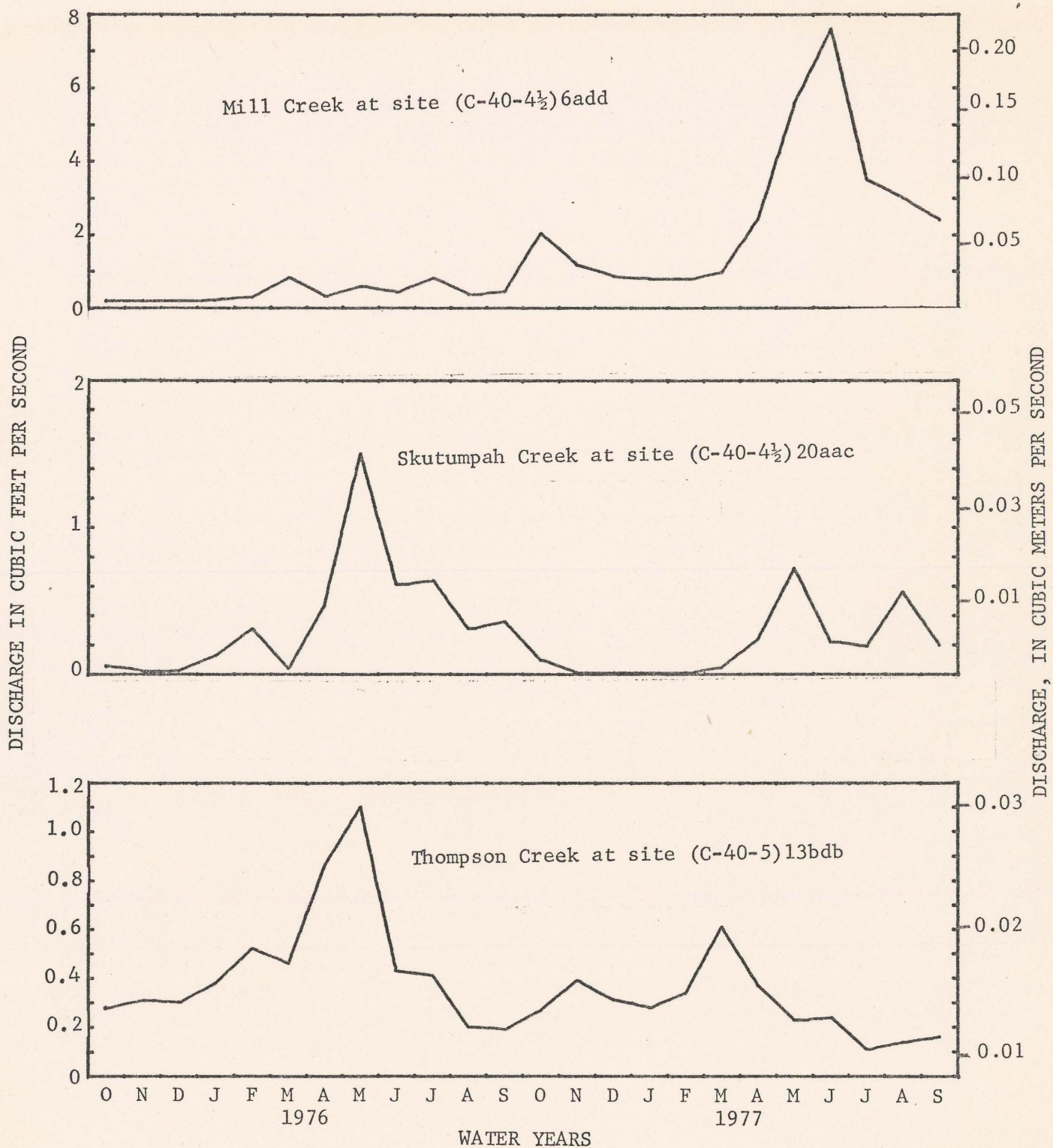
Figure 7.--Streamflow hydrographs of Mill, Skutumpah, and Thompson Creeks, 1976 and 1977 water years.
