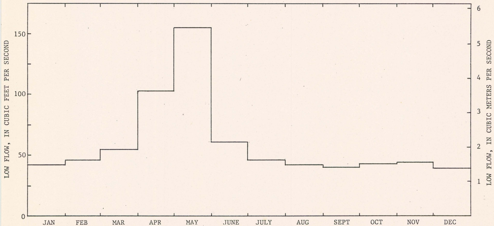
Figure 8.--Estimated average monthly low flow (1937-76) of the North Fork Virgin River at site (C-41-10)22bc.
