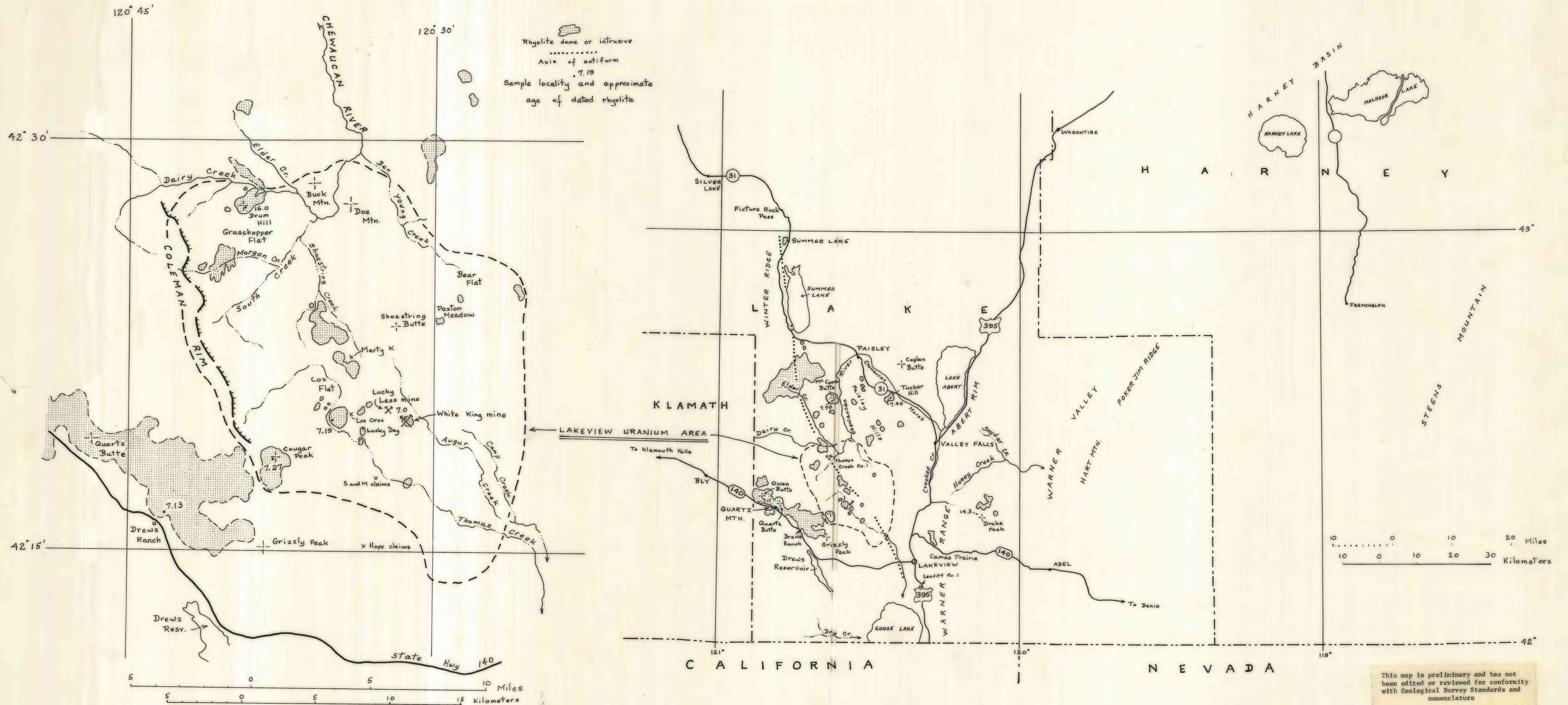
Figure 2.- Index to geographic localities of region, rhyolite sample localities for which isotopic dates are available, and distribution of rhyolite domes and intrusives
