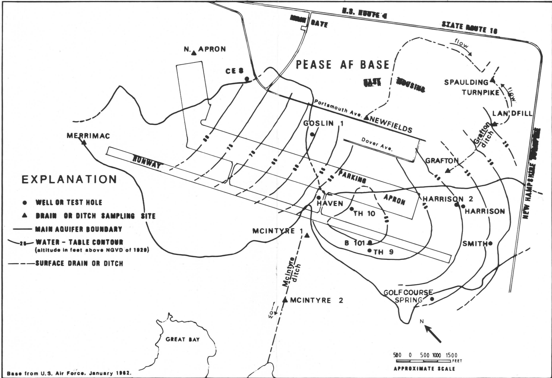
Figure 1.-- Main aquifer, water table contours, and selected data sampling sites.
