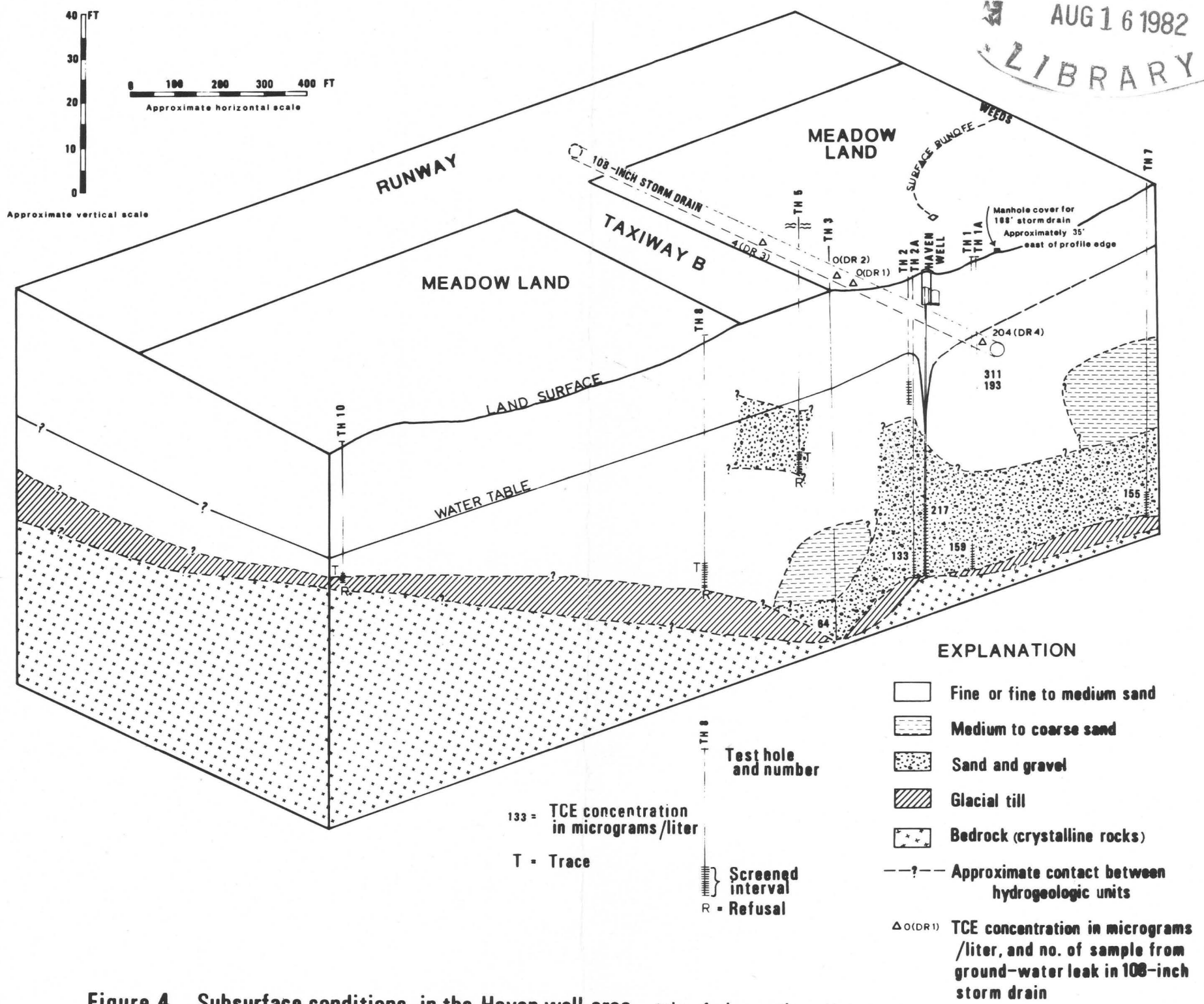
Figure 4. Subsurface conditions in the Haven well area (view facing northwest)
