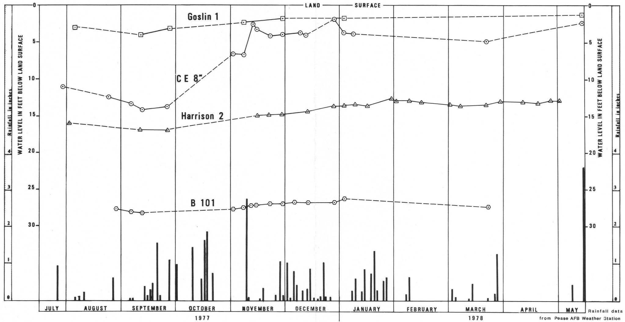
Figure 5.— Daily rainfall (snowfall not included) and water-level fluctuation in selected observation wells, 1977-78
