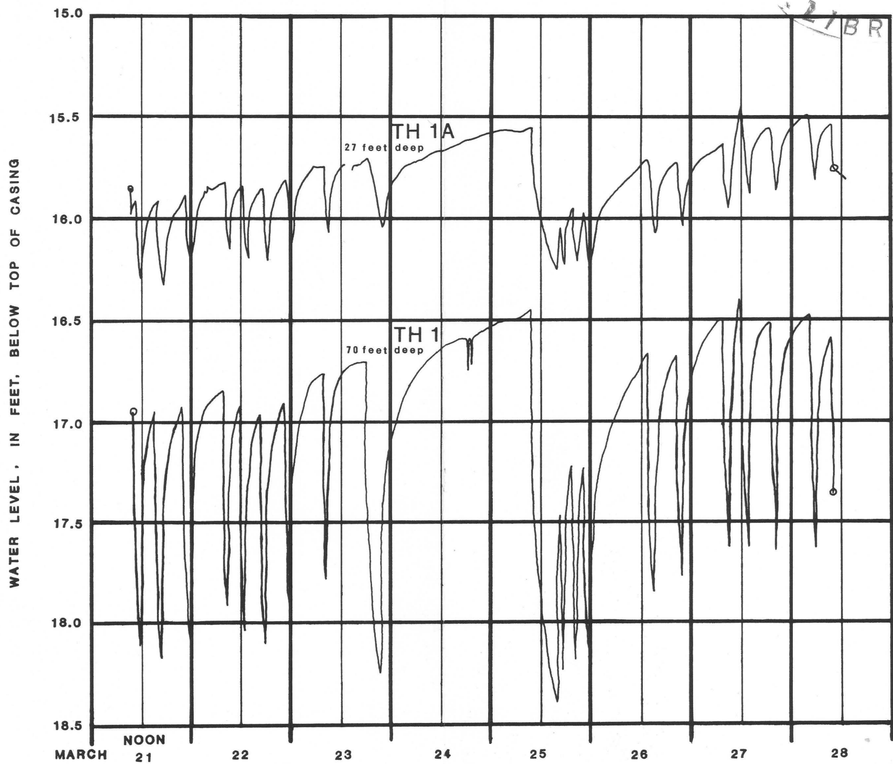
Figure 6.--Water-level fluctuations in test holes TH 1 and TH 1A, March 21-28, 1978
