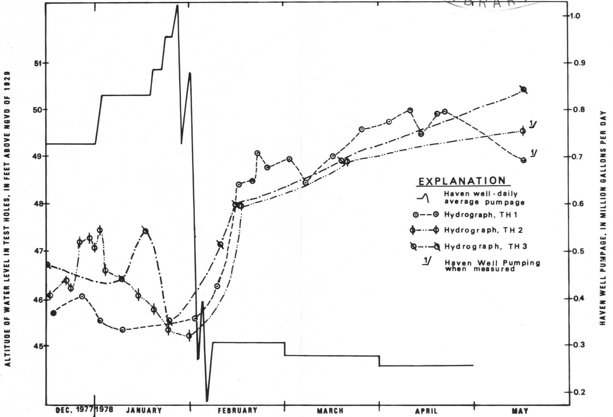
Figure 7.-- Comparison of pumpage at Haven well and water levels in nearby test holes
