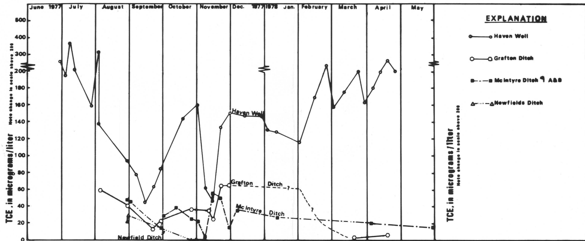
FIGURE 8. --Fluctuations in TCE concentration at Haven well and at selected ditch sampling sites, 1977-1978
