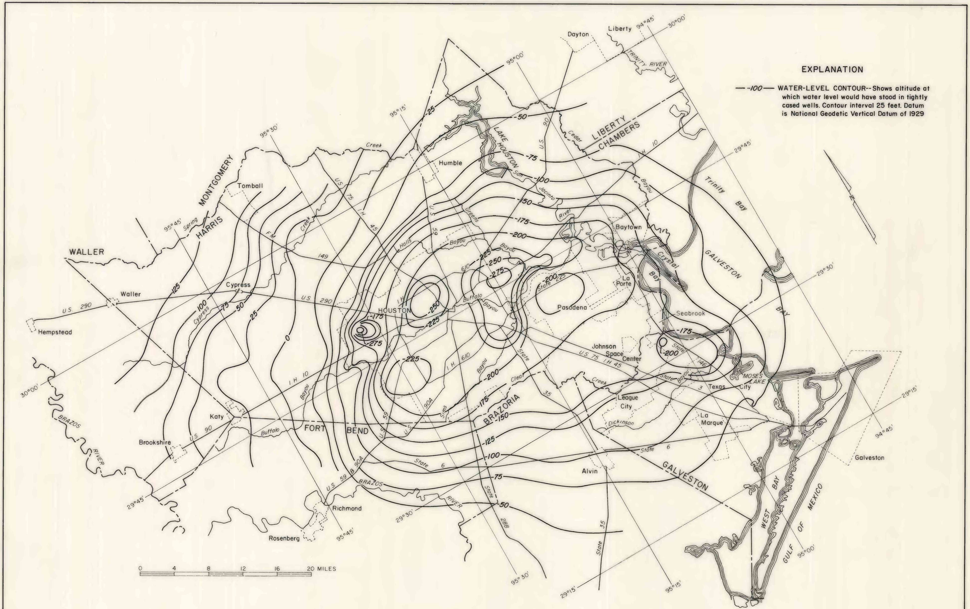
FIGURE 2.—Approximate altitude of water levels in wells in the Chicot aquifer, Spring 1980
