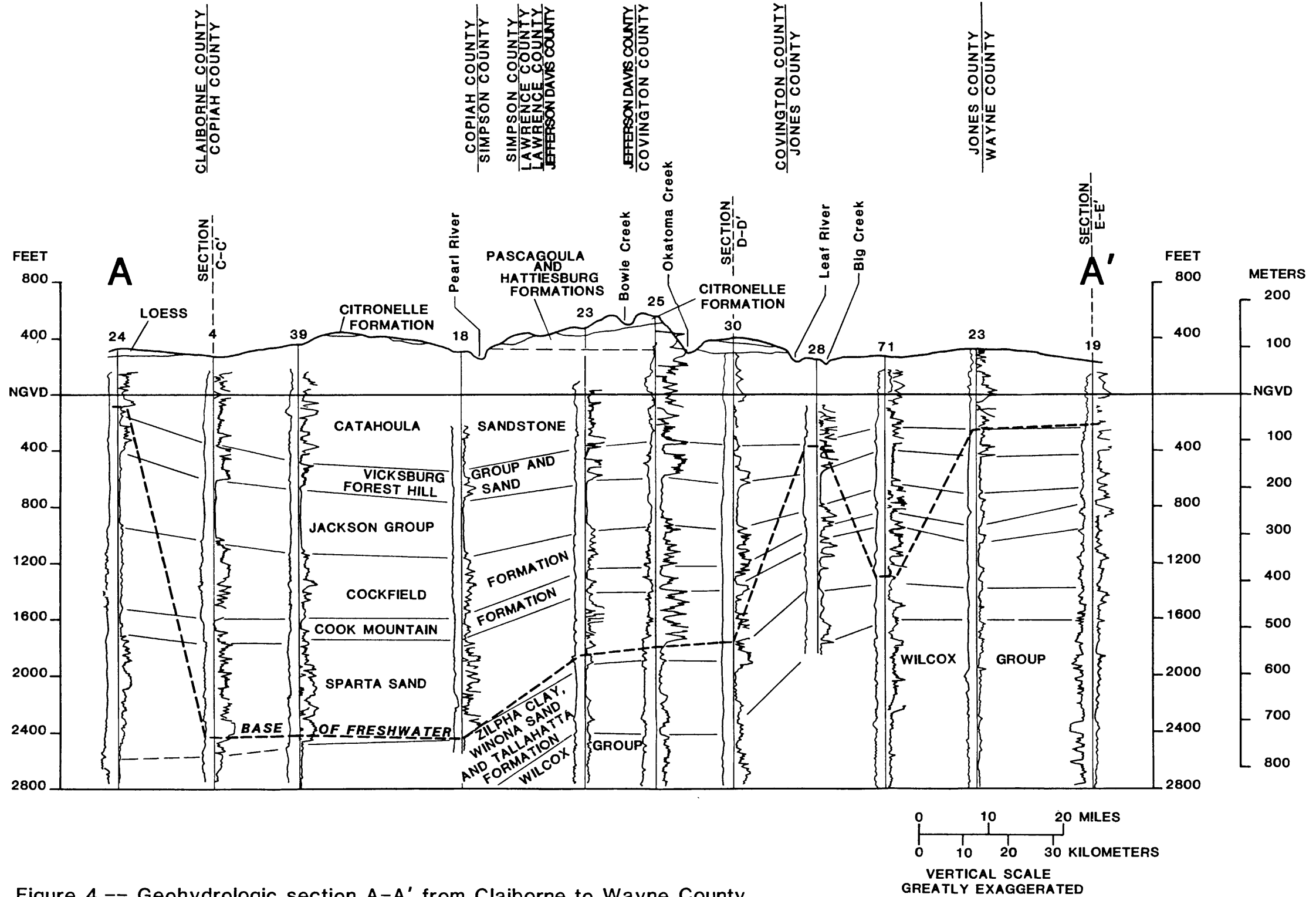
Figure 4.-- Geohydrologic section A-A' from Claiborne to Wayne County.
