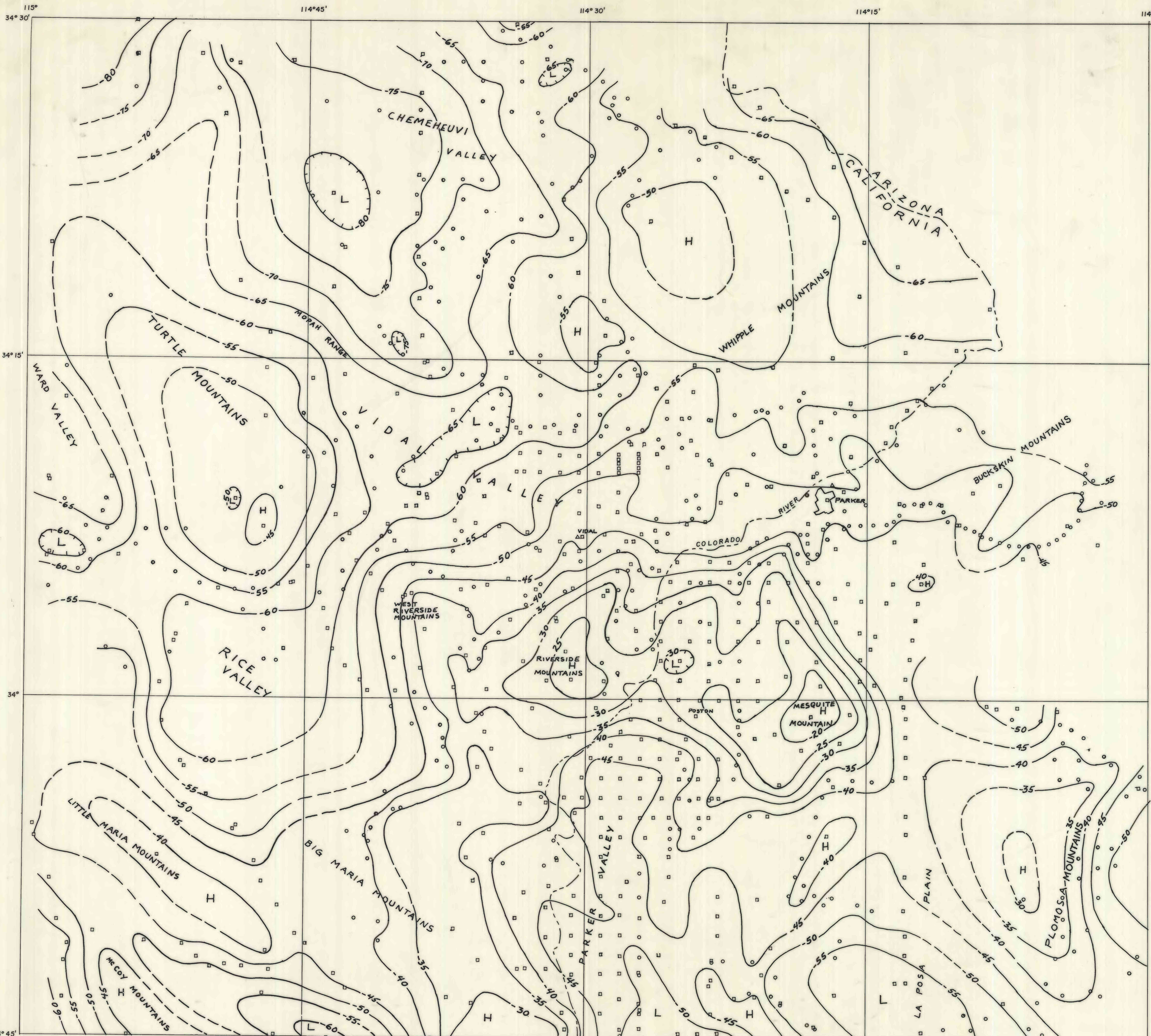
Complete Bouguer gravity map of the Vidal area, California and Arizona compiled by D.L. Healey and F.E. Currey
